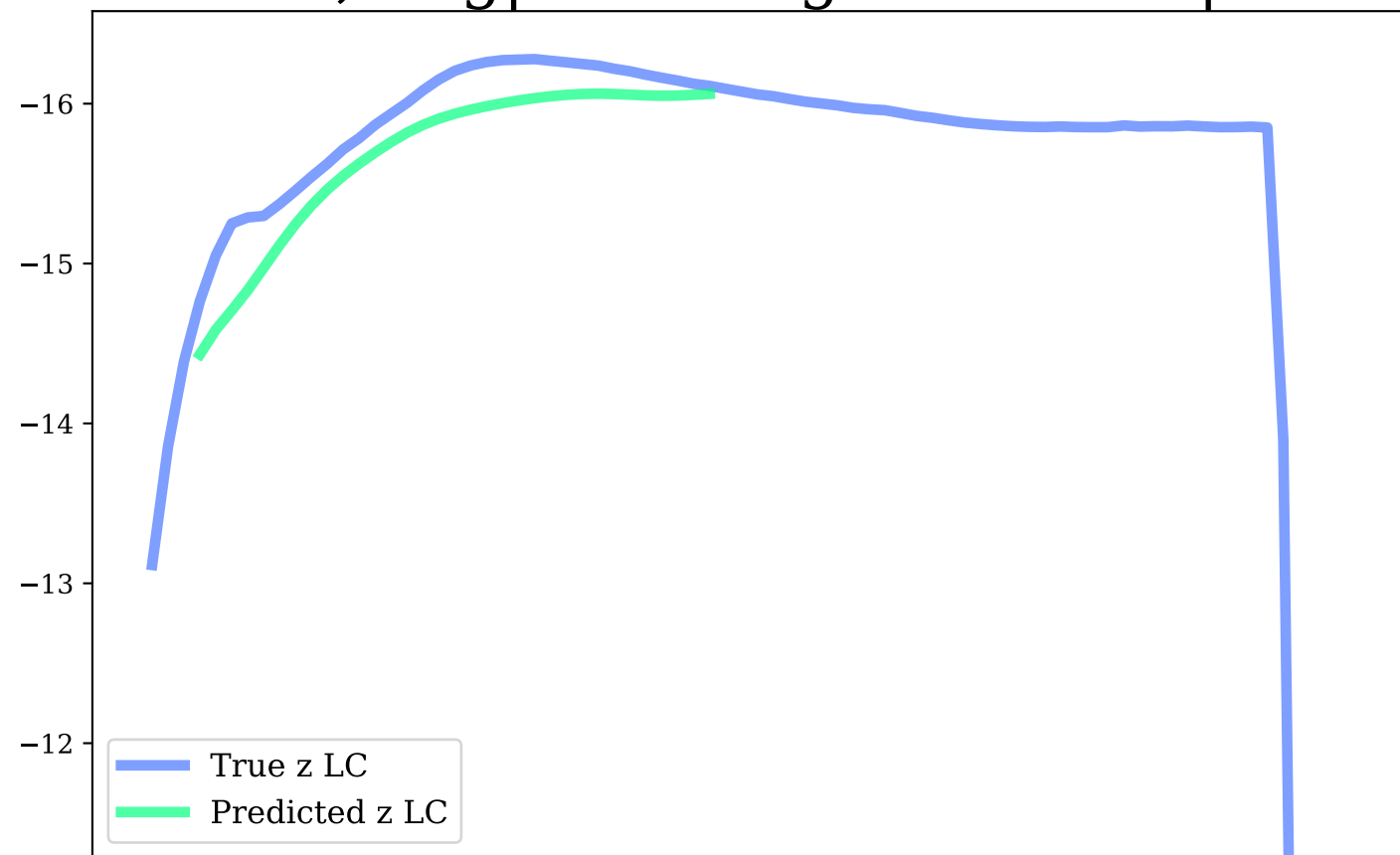
z-band, Avg|Max Mag Diff: 0.22 | 0.54
