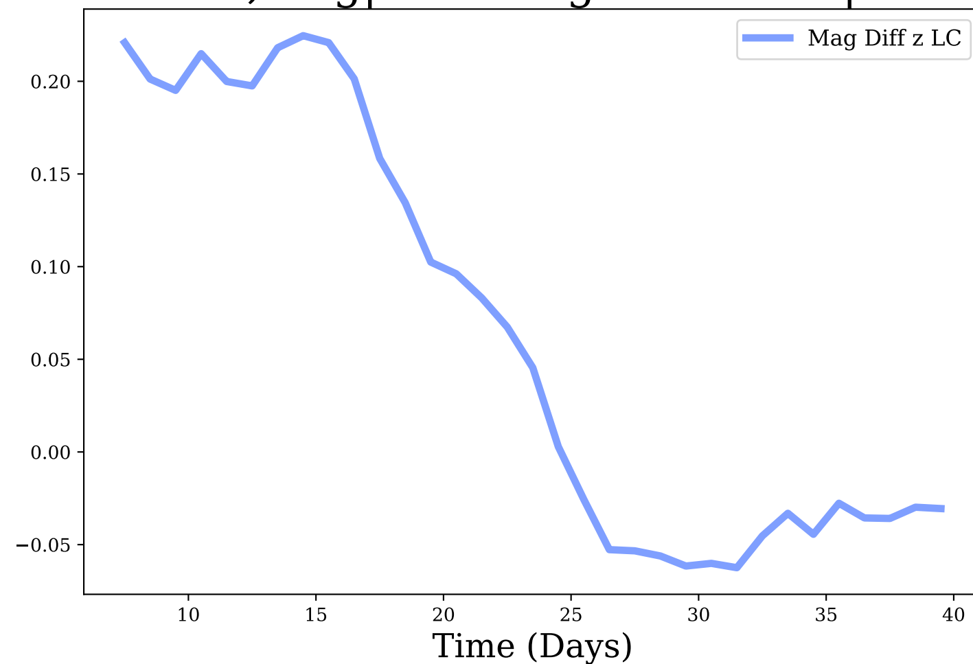
z-band, Avg|Max Mag Diff: 0.06 | 0.22
