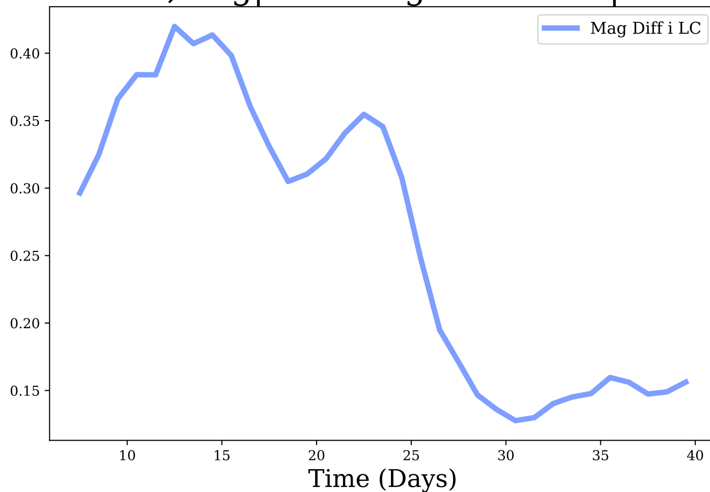
i-band, Avg|Max Mag Diff: 0.26 | 0.42
