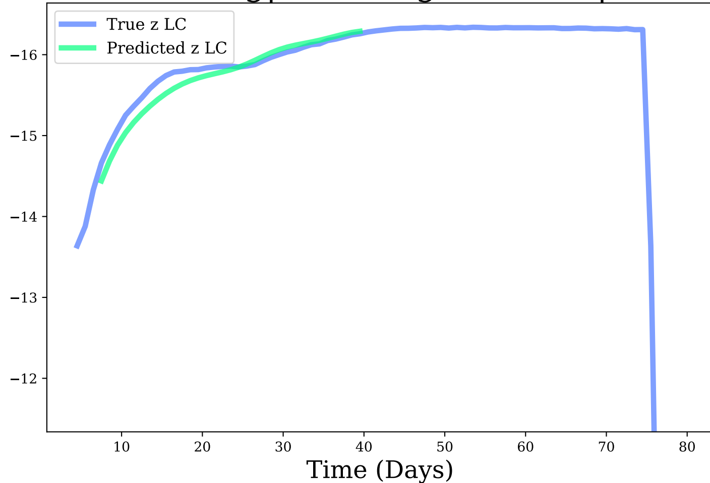
z-band, Avg|Max Mag Diff: 0.1 | 0.22
