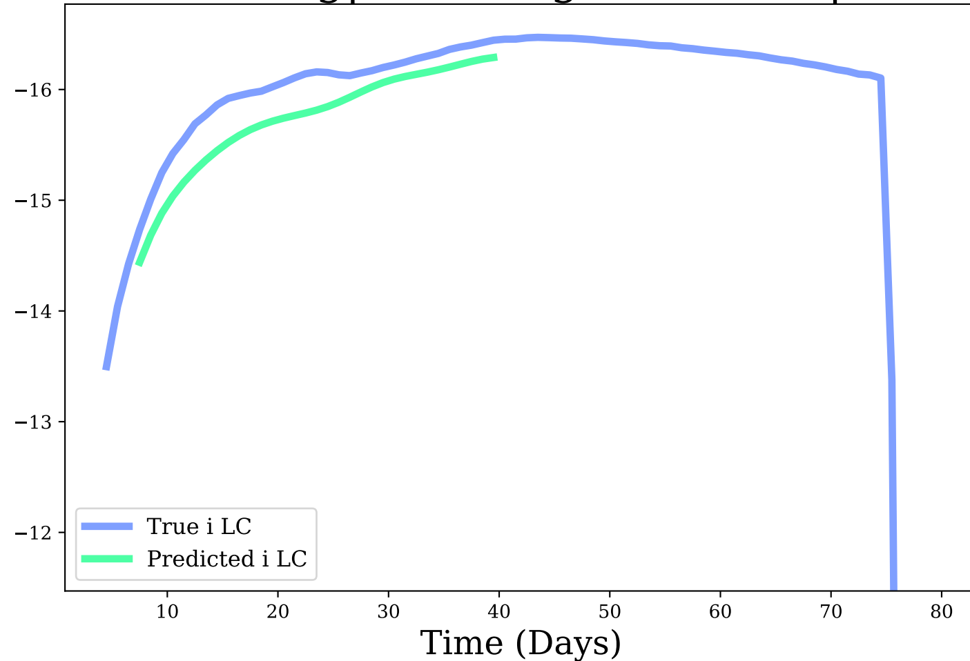
i-band, Avg|Max Mag Diff: 0.26 | 0.42
