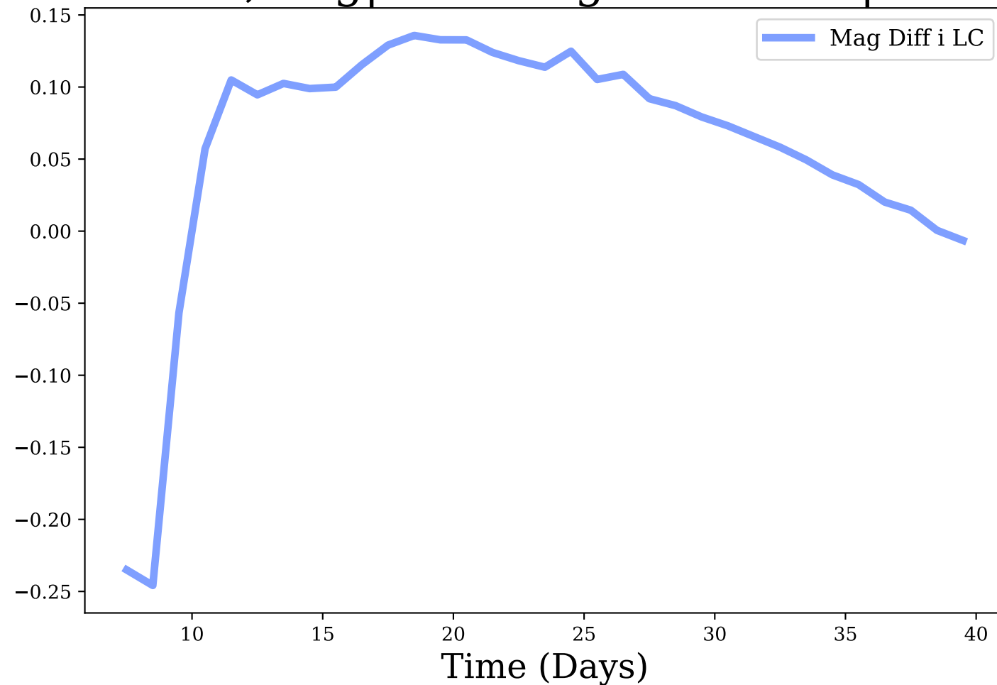
i-band, Avg|Max Mag Diff: 0.06 | 0.25
