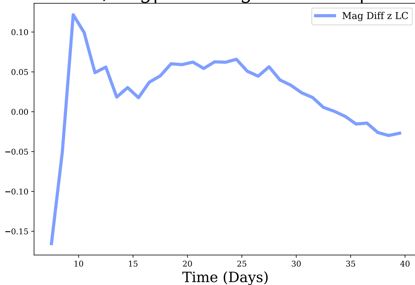
z-band, Avg|Max Mag Diff: 0.03 | 0.17
