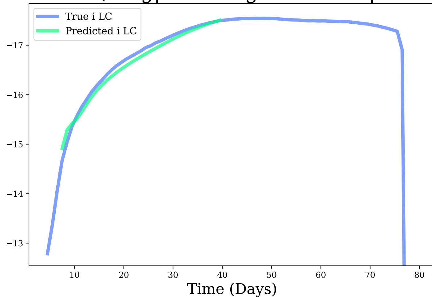
i-band, Avg|Max Mag Diff: 0.09 | 0.25
