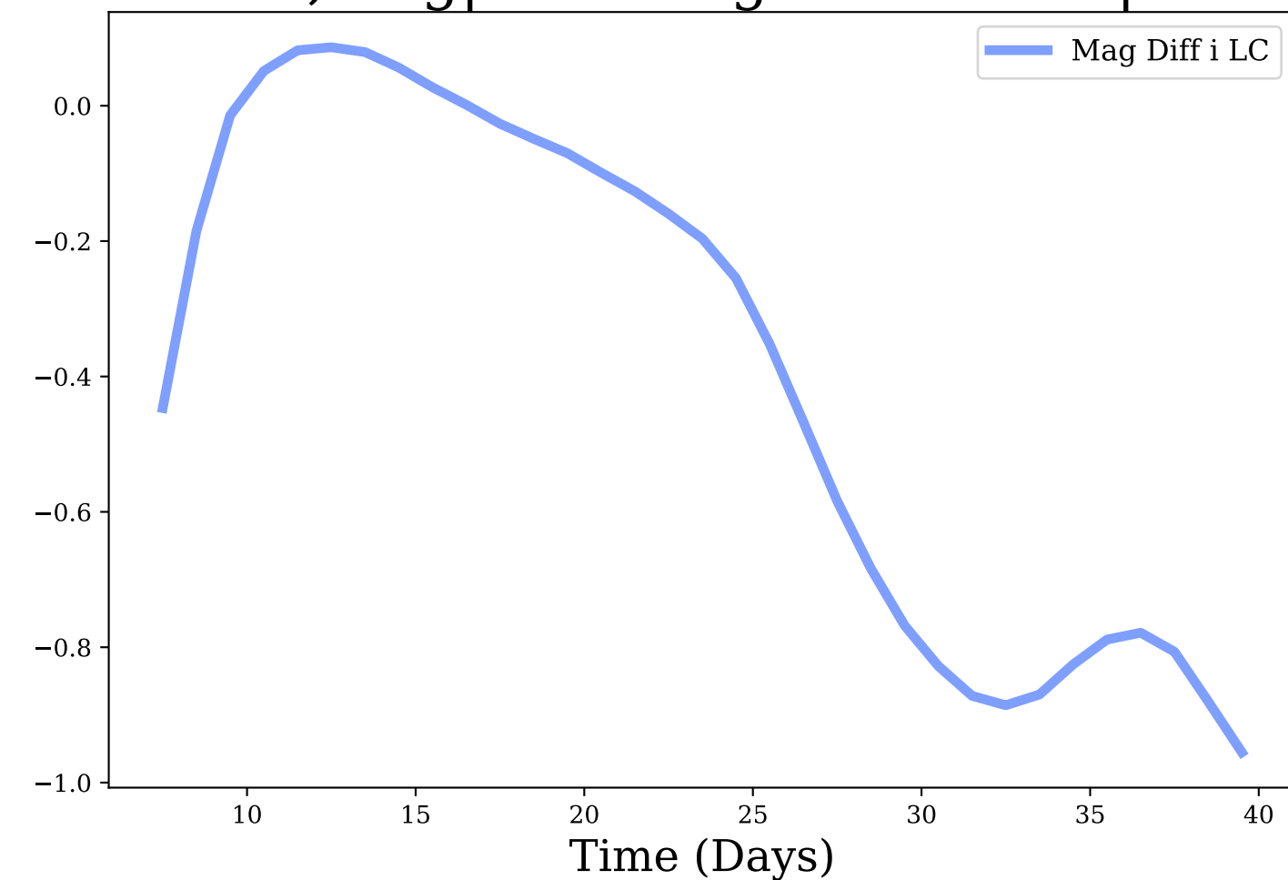
i-band, Avg|Max Mag Diff: -0.38 | 0.96
