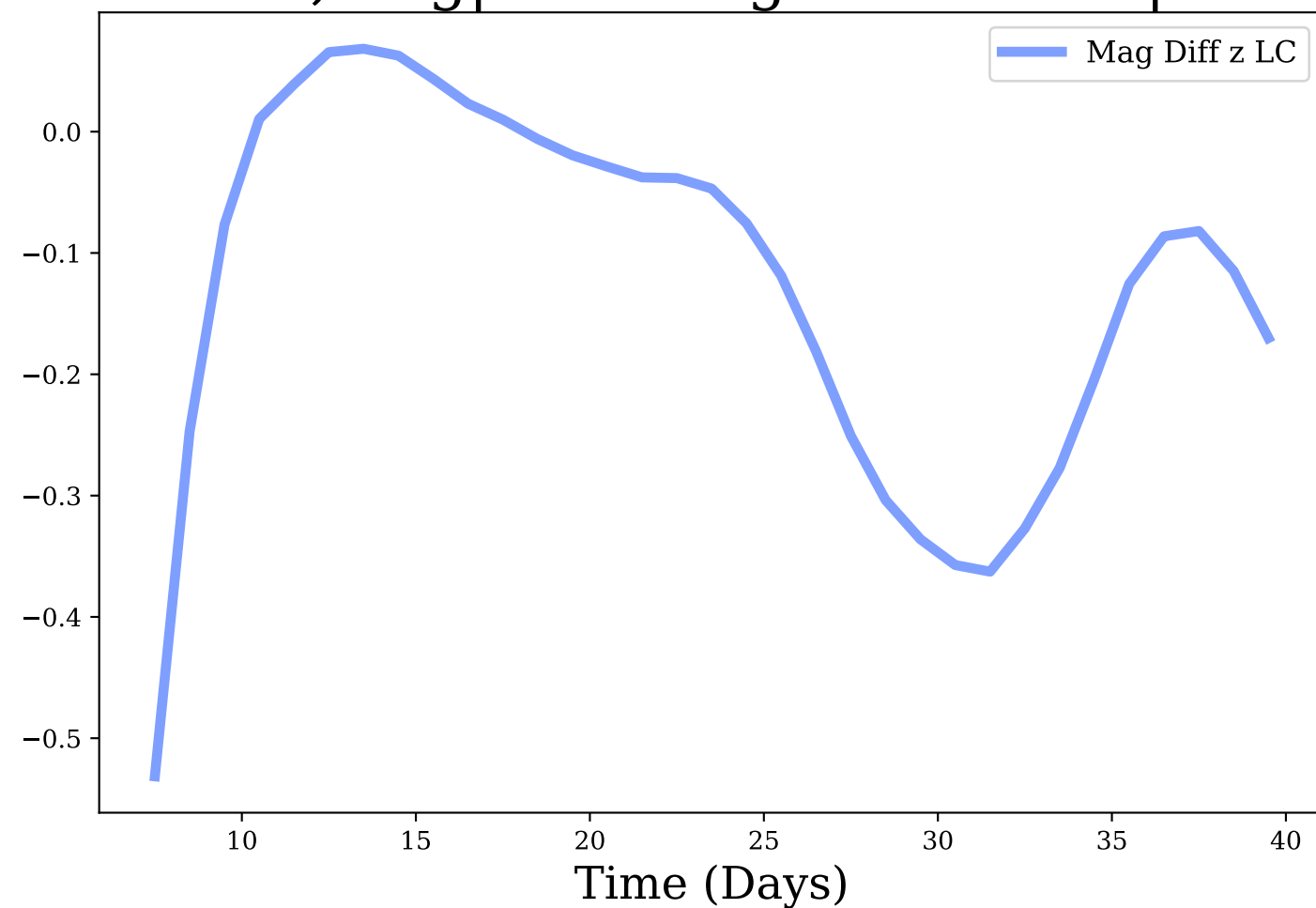
z-band, Avg|Max Mag Diff: -0.12 | 0.53
