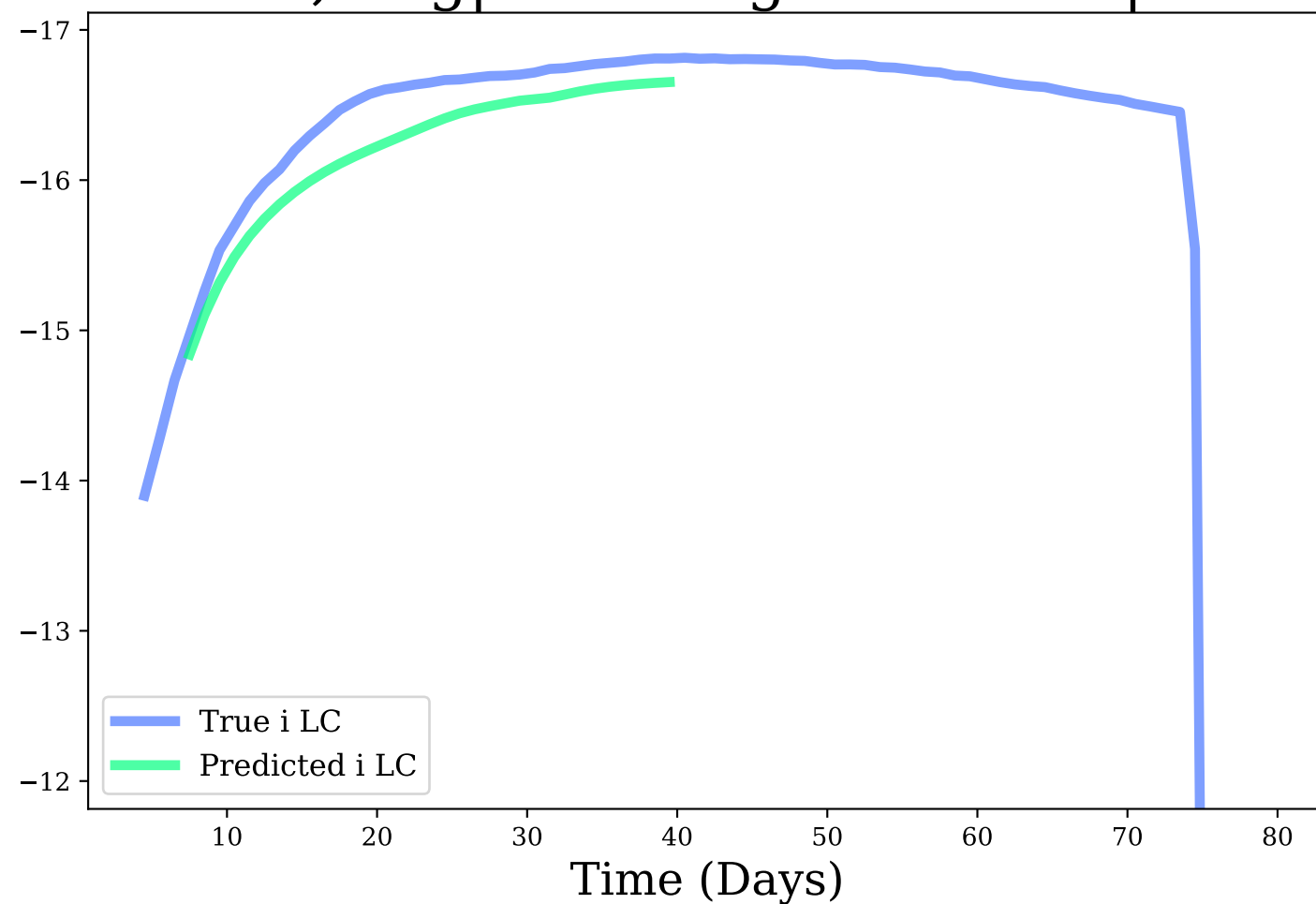
i-band, Avg|Max Mag Diff: 0.23 | 0.37
