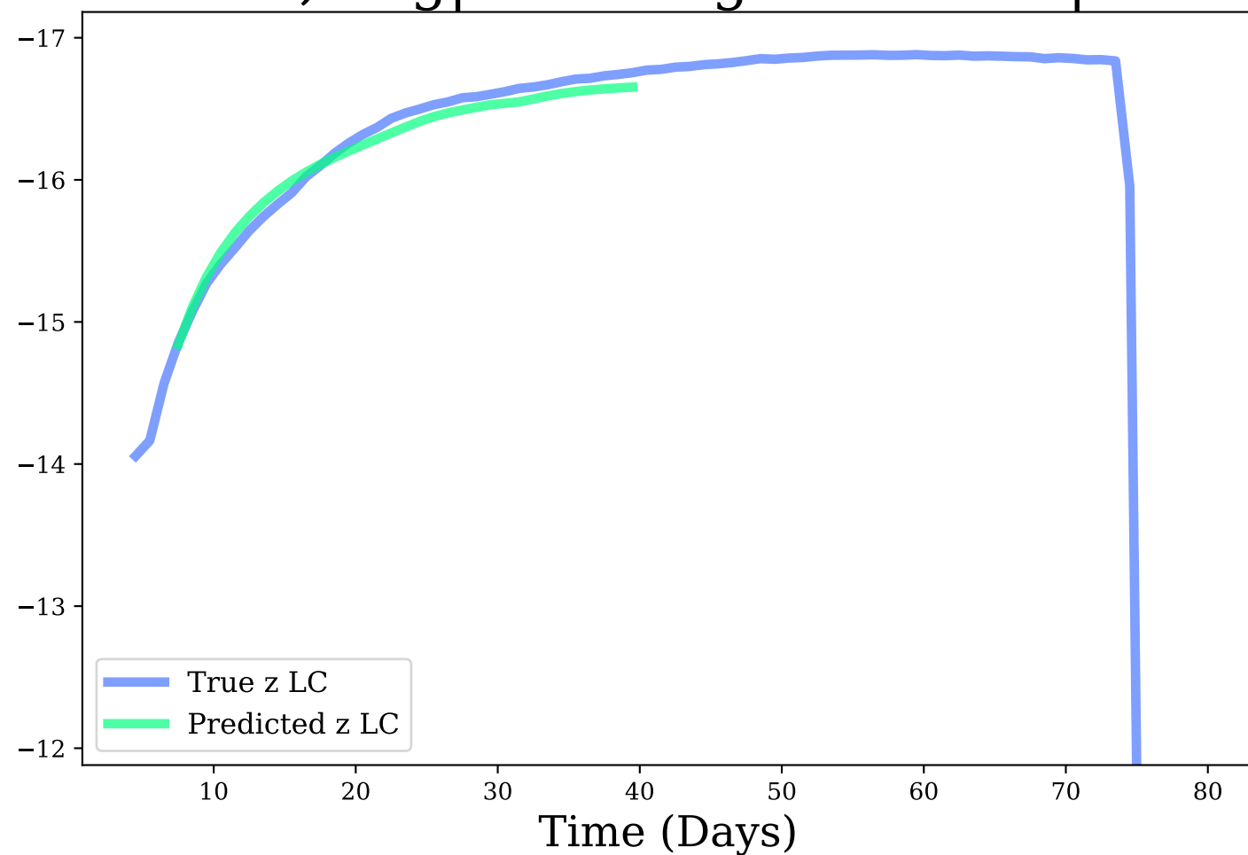
z-band, Avg|Max Mag Diff: 0.08 | 0.11
