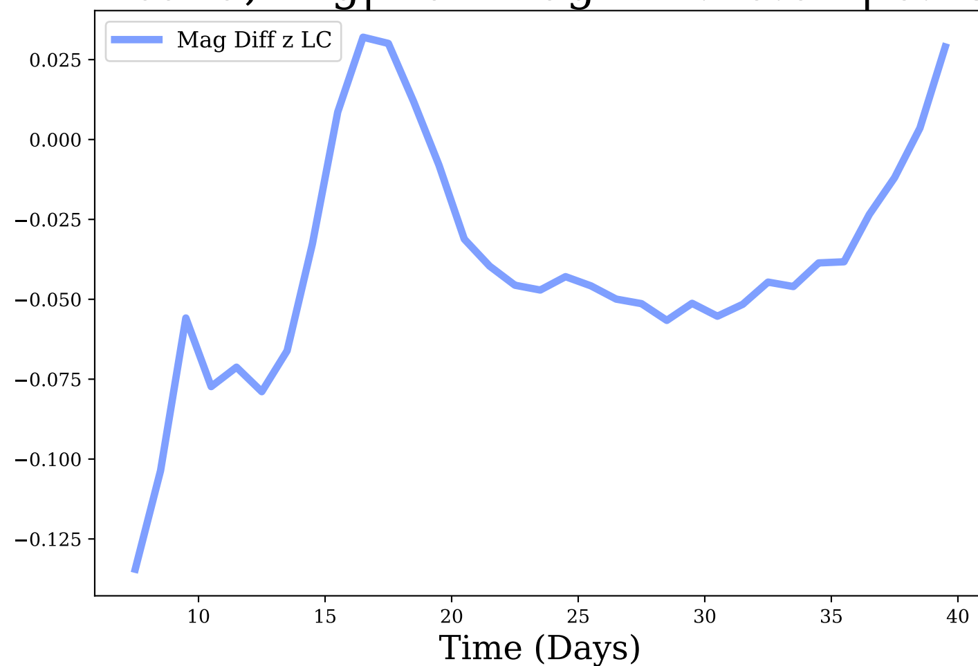
z-band, Avg|Max Mag Diff: -0.04 | 0.13
