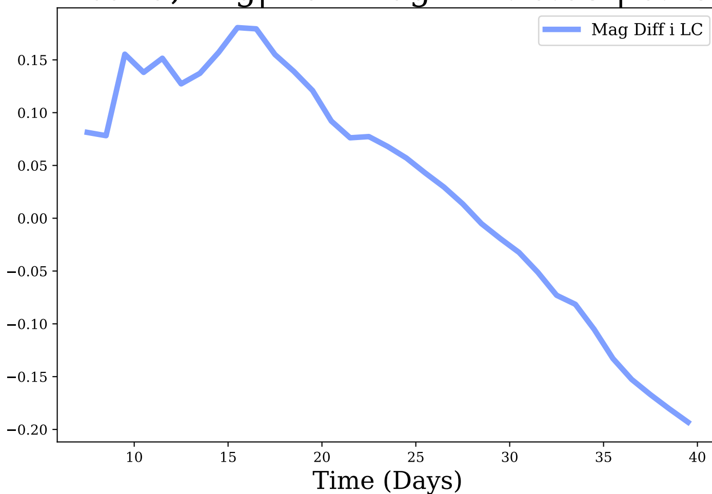
i-band, Avg|Max Mag Diff: 0.03 | 0.19
