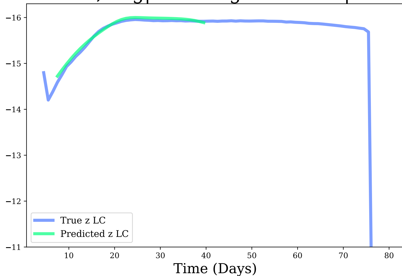
z-band, Avg|Max Mag Diff: 0.05 | 0.13
