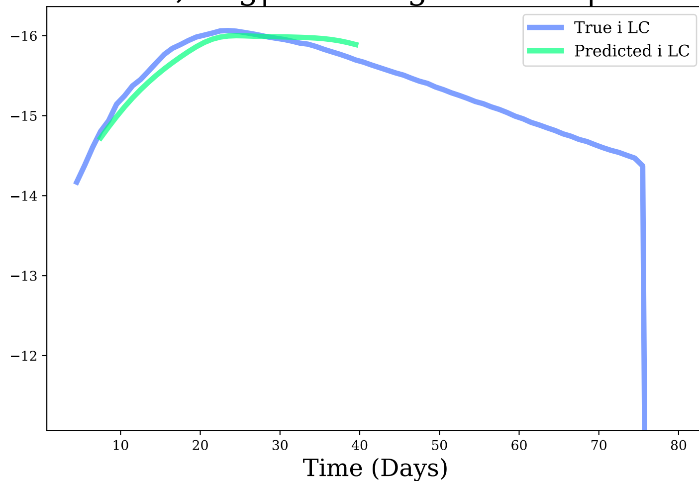
i-band, Avg|Max Mag Diff: 0.1 | 0.19
