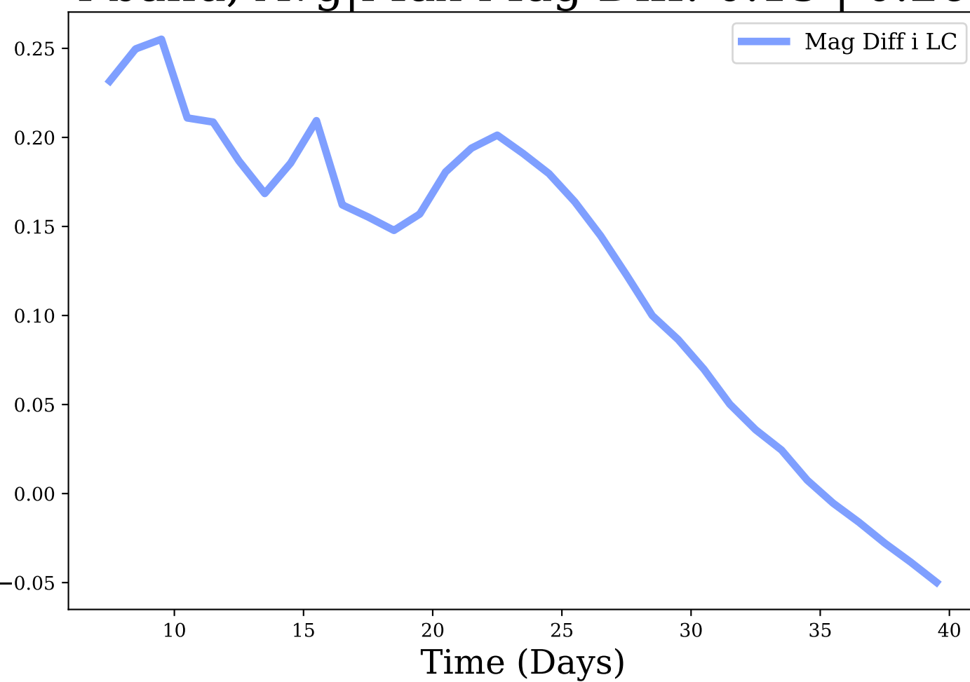
i-band, Avg|Max Mag Diff: 0.13 | 0.26
