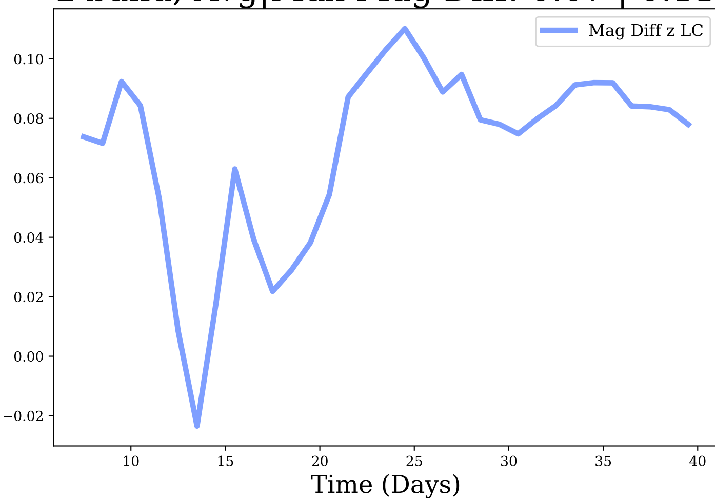
z-band, Avg|Max Mag Diff: 0.07 | 0.11
