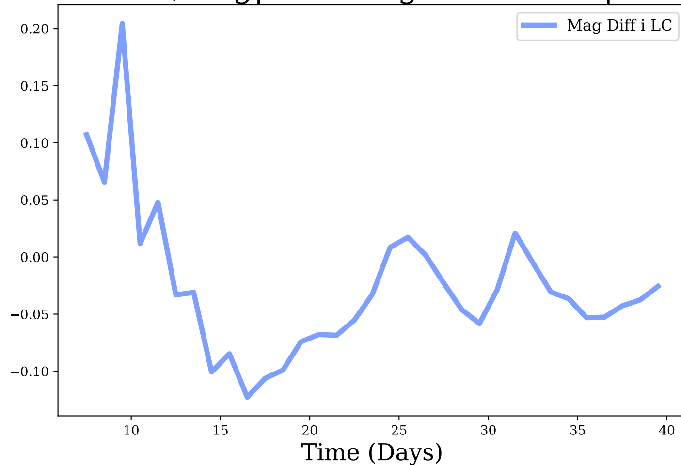
i-band, Avg|Max Mag Diff: -0.03 | 0.2
