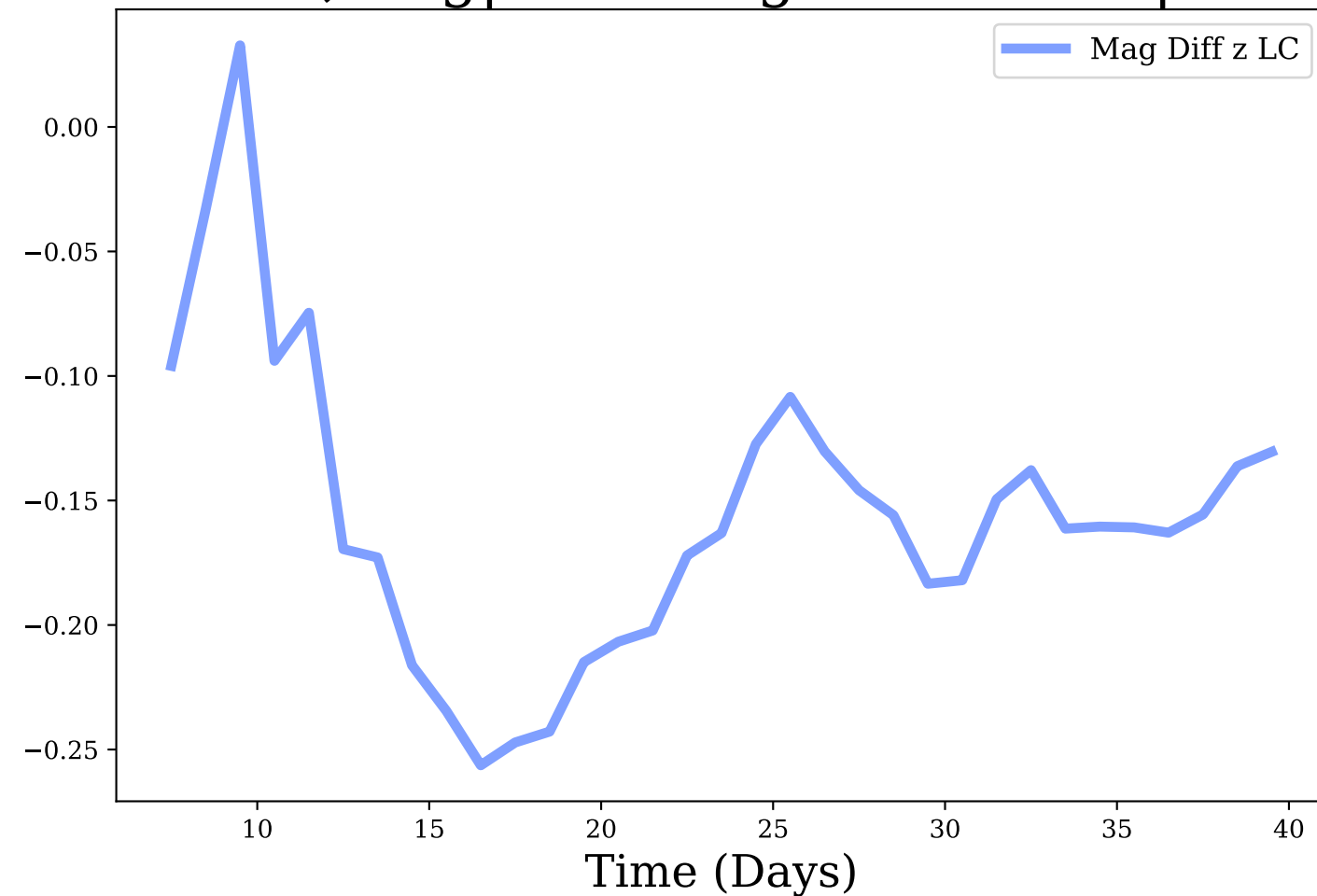
z-band, Avg|Max Mag Diff: -0.16 | 0.26
