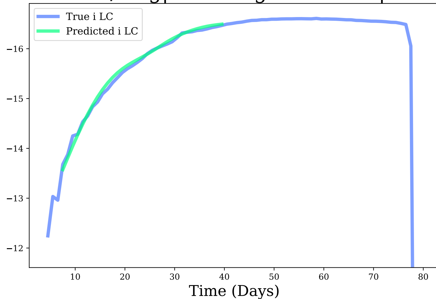
i-band, Avg|Max Mag Diff: 0.05 | 0.2
