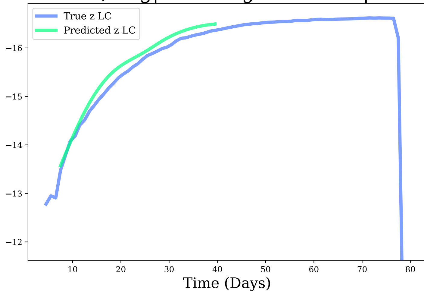
z-band, Avg|Max Mag Diff: 0.16 | 0.26
