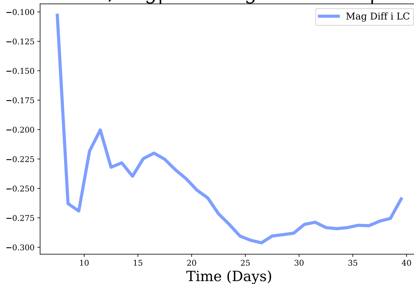
i-band, Avg|Max Mag Diff: -0.26 | 0.3
