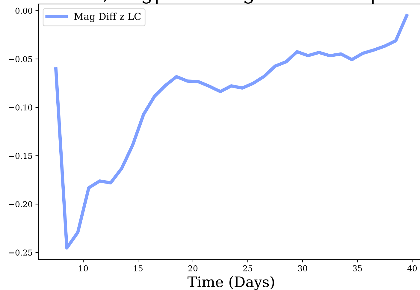
z-band, Avg|Max Mag Diff: -0.09 | 0.25
