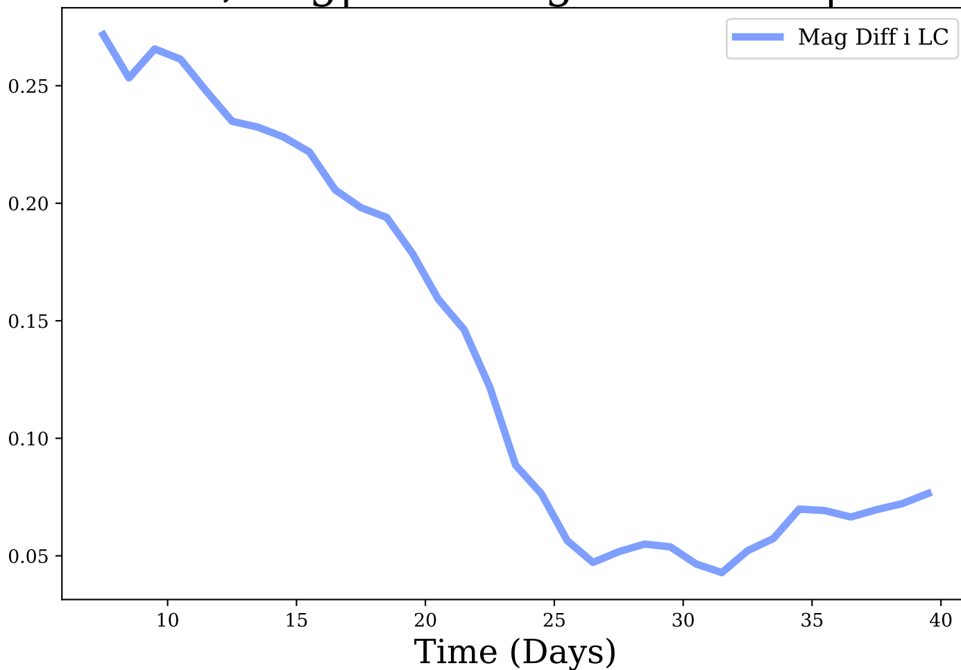
i-band, Avg|Max Mag Diff: 0.14 | 0.27
