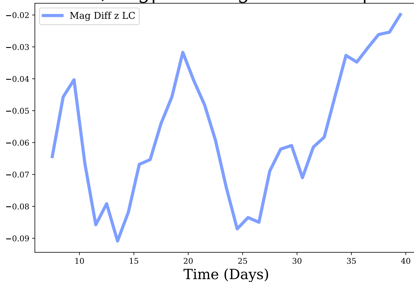
z-band, Avg|Max Mag Diff: -0.06 | 0.09
