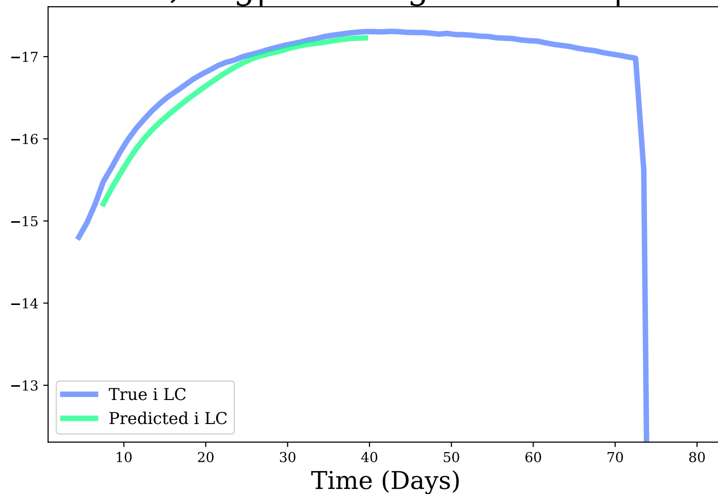
i-band, Avg|Max Mag Diff: 0.14 | 0.27
