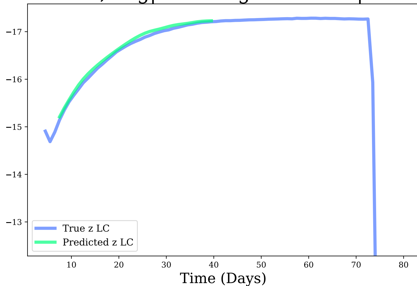
z-band, Avg|Max Mag Diff: 0.06 | 0.09
