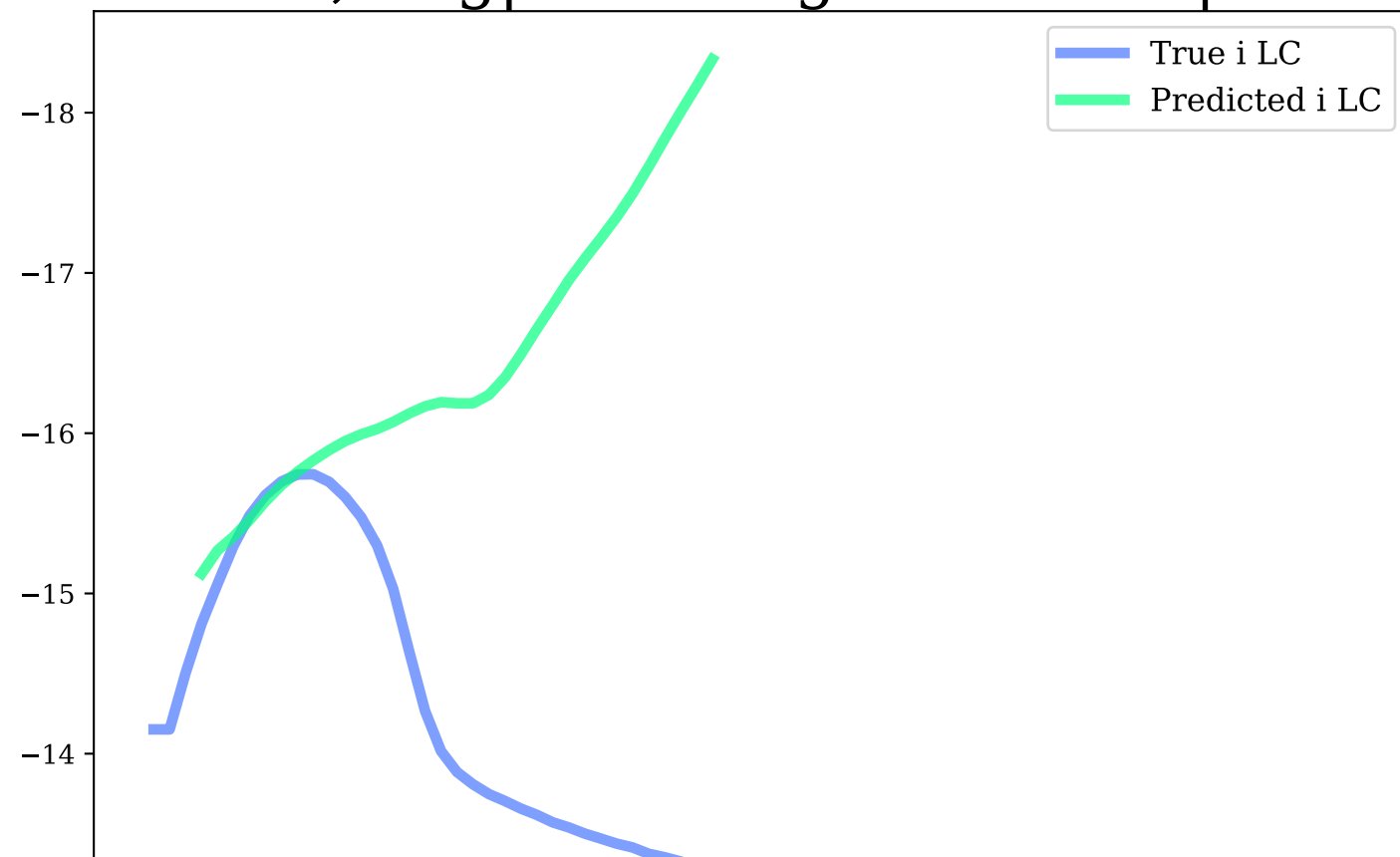
i-band, Avg|Max Mag Diff: 2.13 | 5.07
