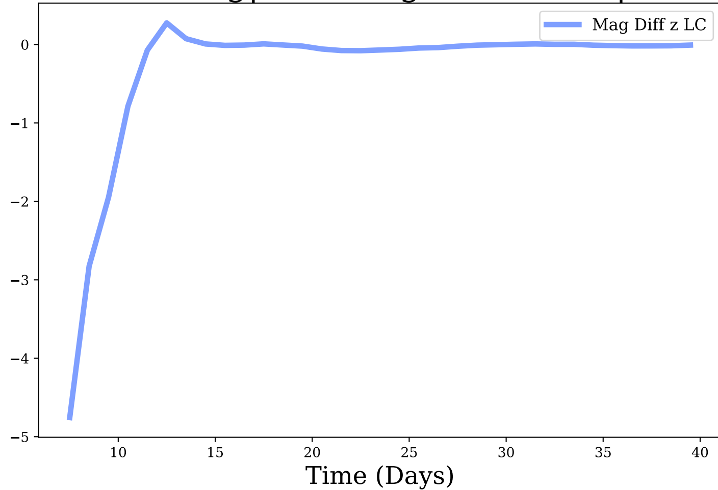
z-band, Avg|Max Mag Diff: -0.32 | 4.76
