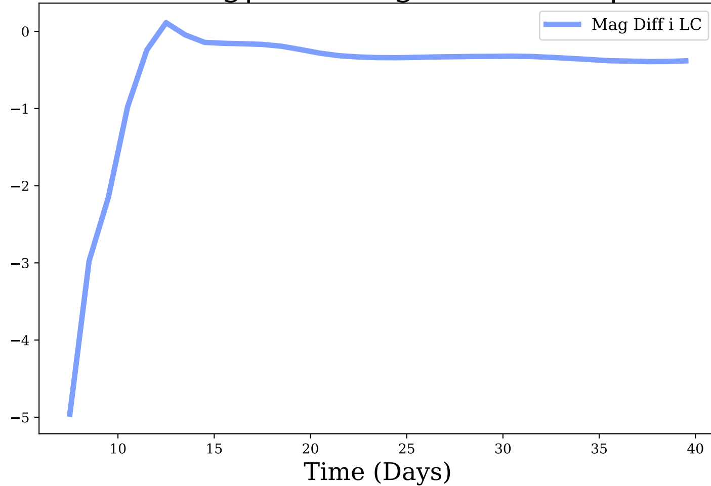
i-band, Avg|Max Mag Diff: -0.58 | 4.96
