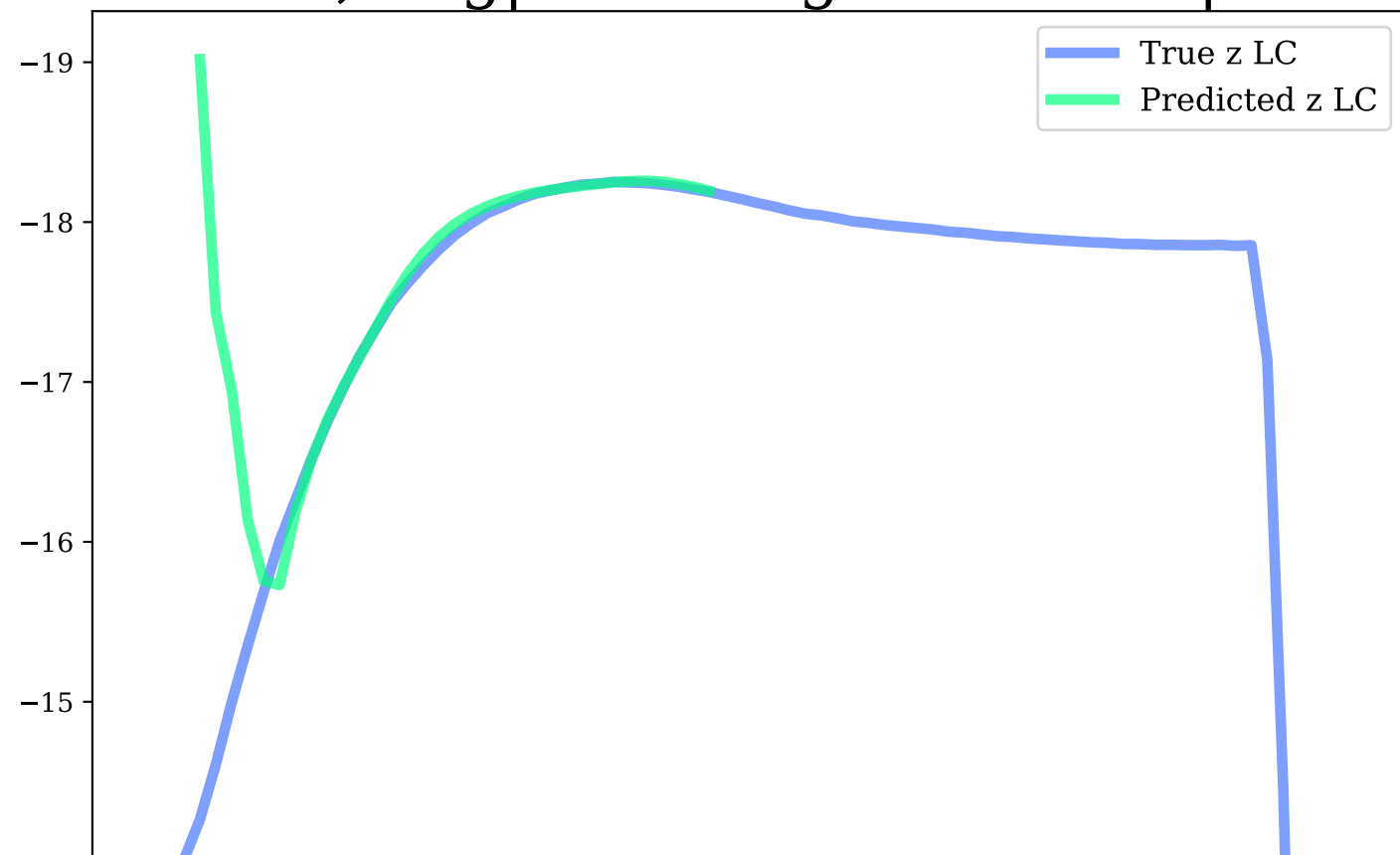
z-band, Avg|Max Mag Diff: 0.34 | 4.76
