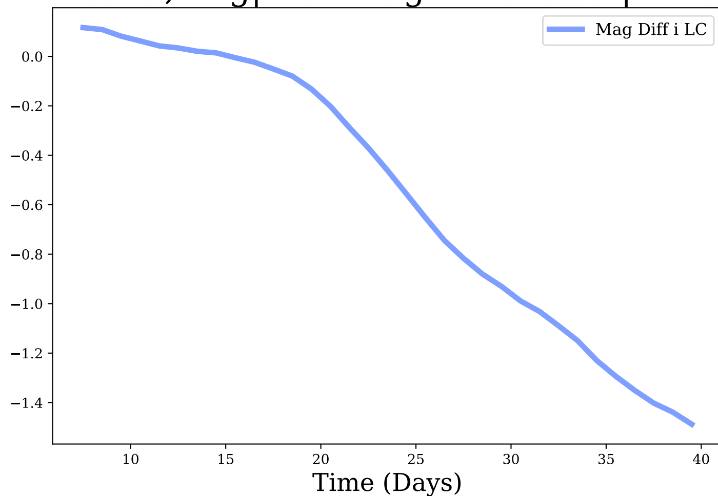
i-band, Avg|Max Mag Diff: -0.55 | 1.49
