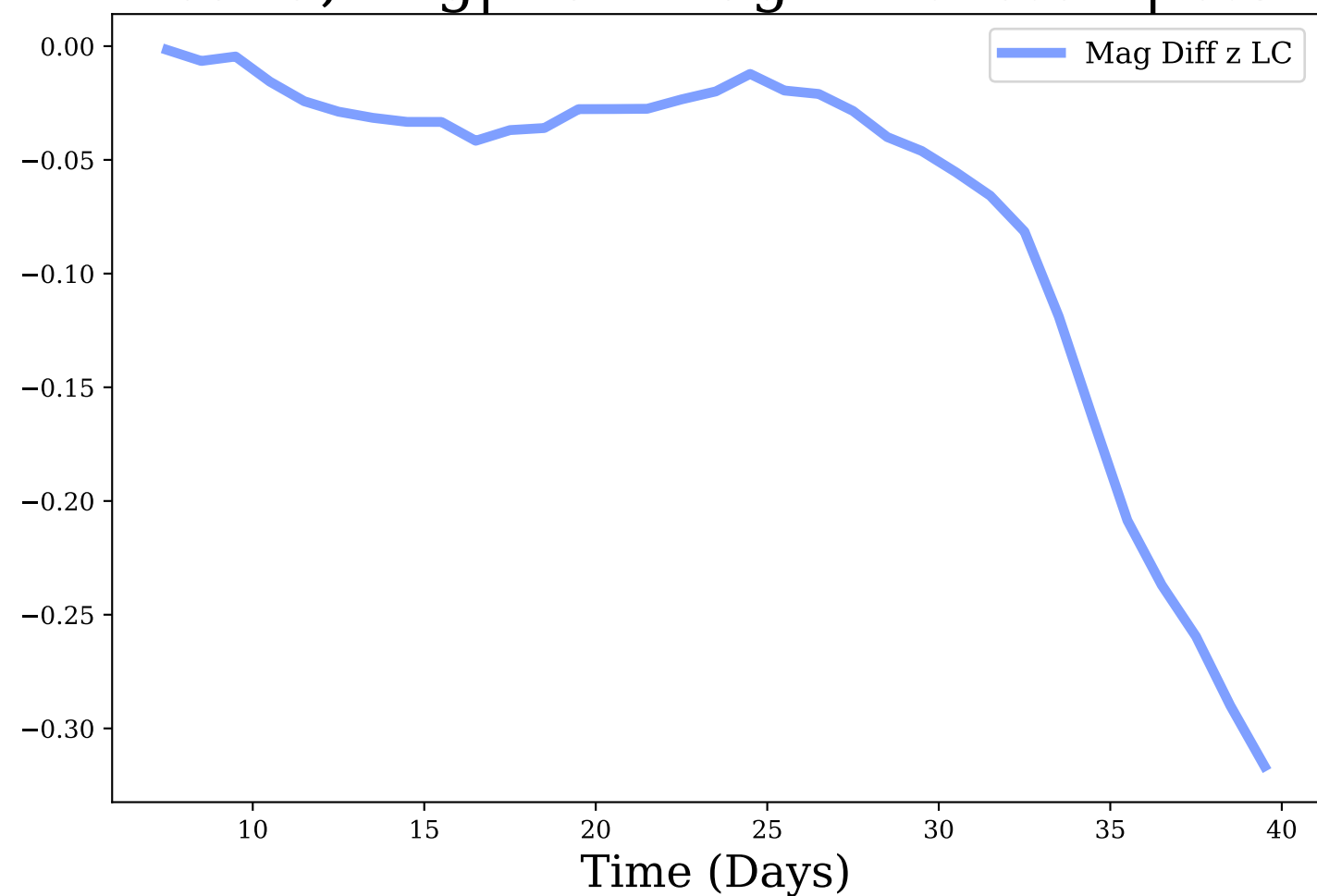
z-band, Avg|Max Mag Diff: -0.07 | 0.32
