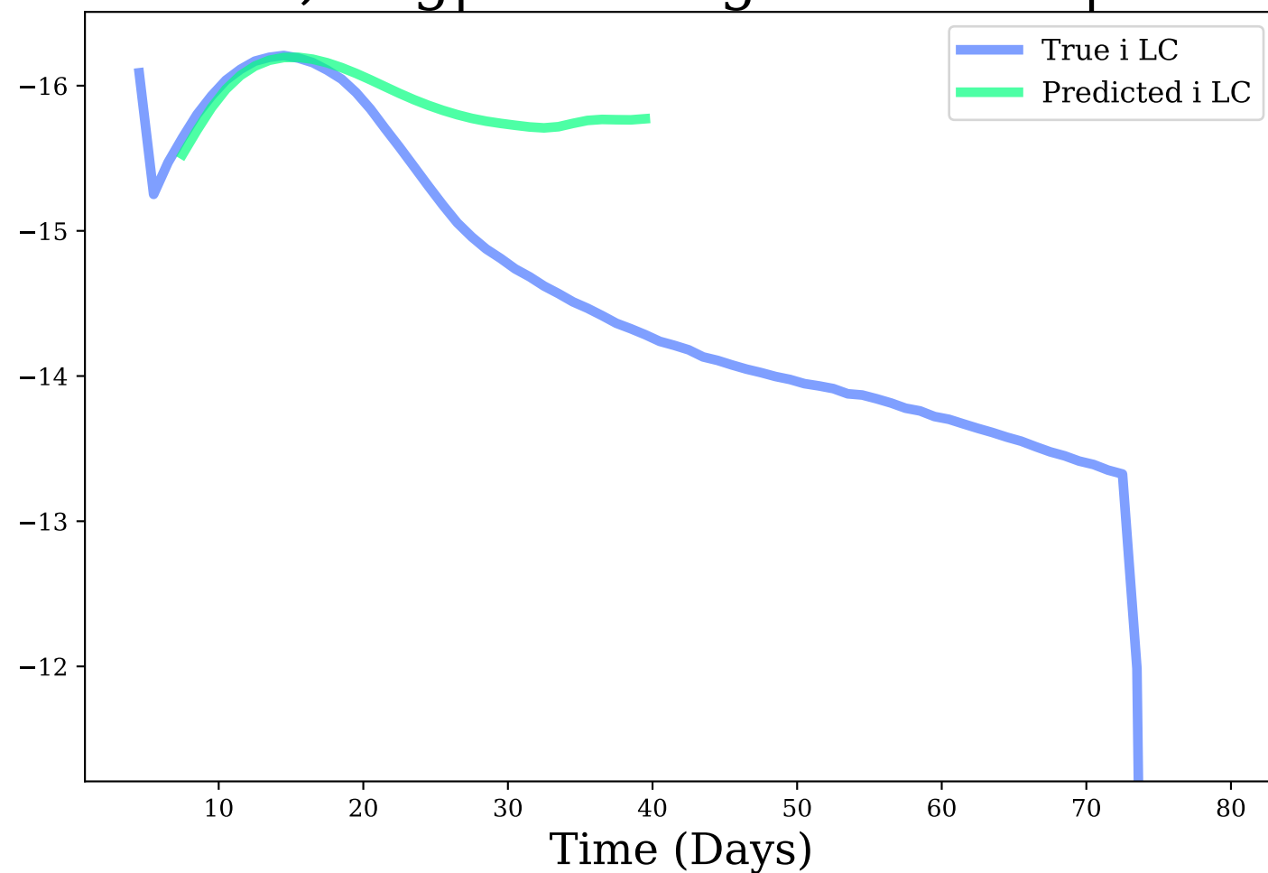
i-band, Avg|Max Mag Diff: 0.58 | 1.49
