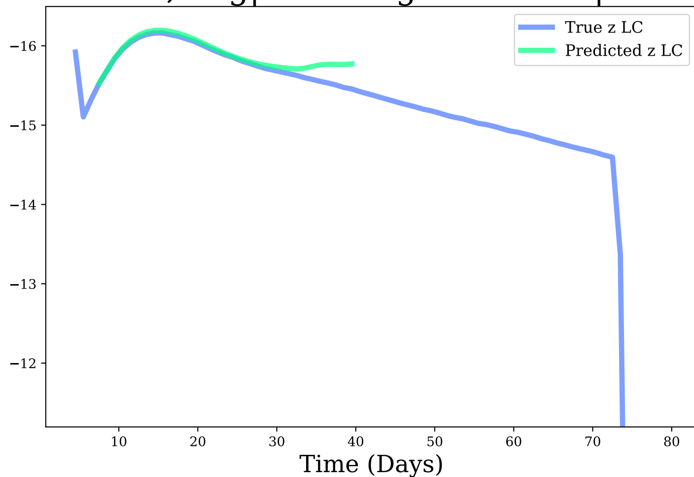
z-band, Avg|Max Mag Diff: 0.07 | 0.32
