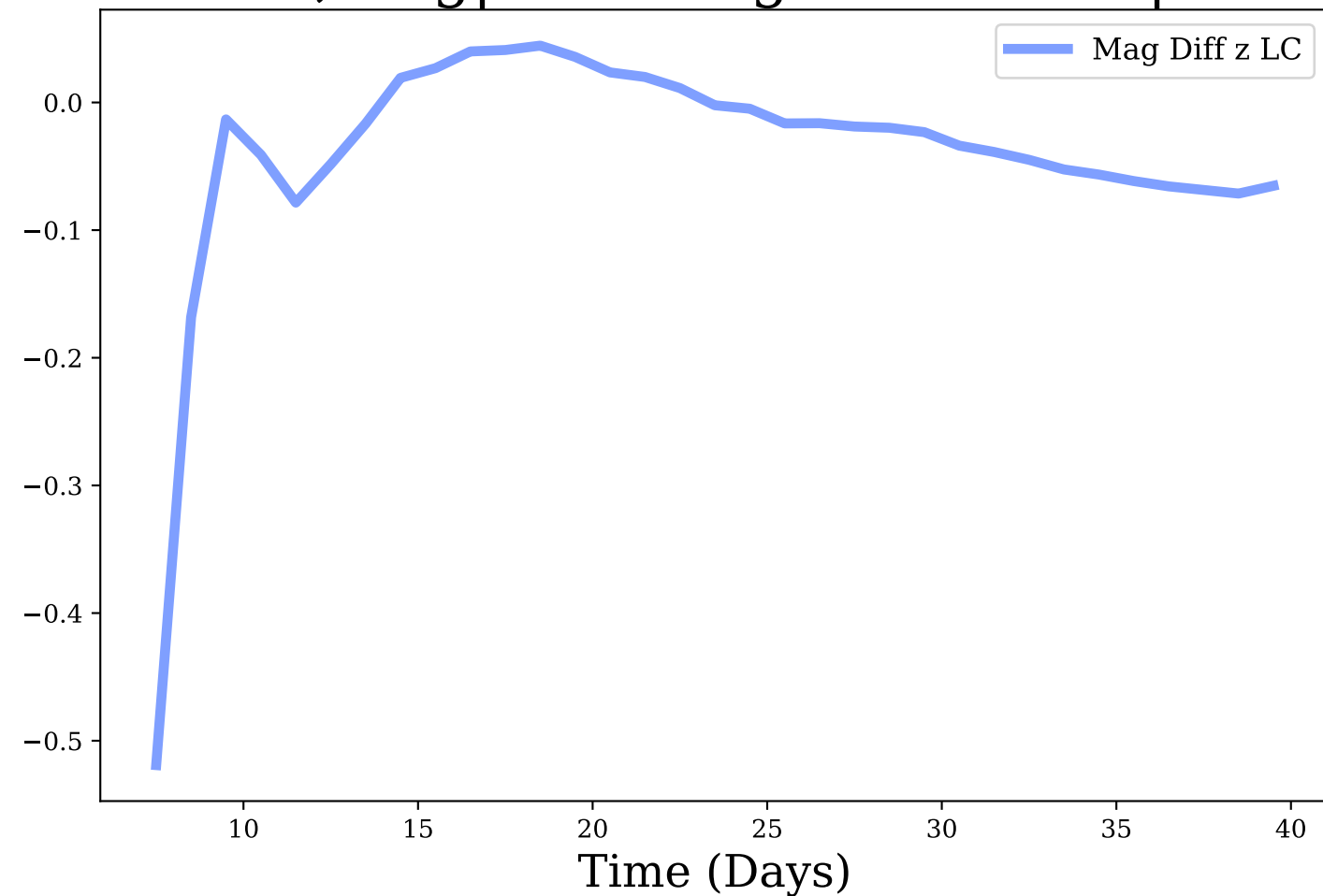
z-band, Avg|Max Mag Diff: -0.04 | 0.52
