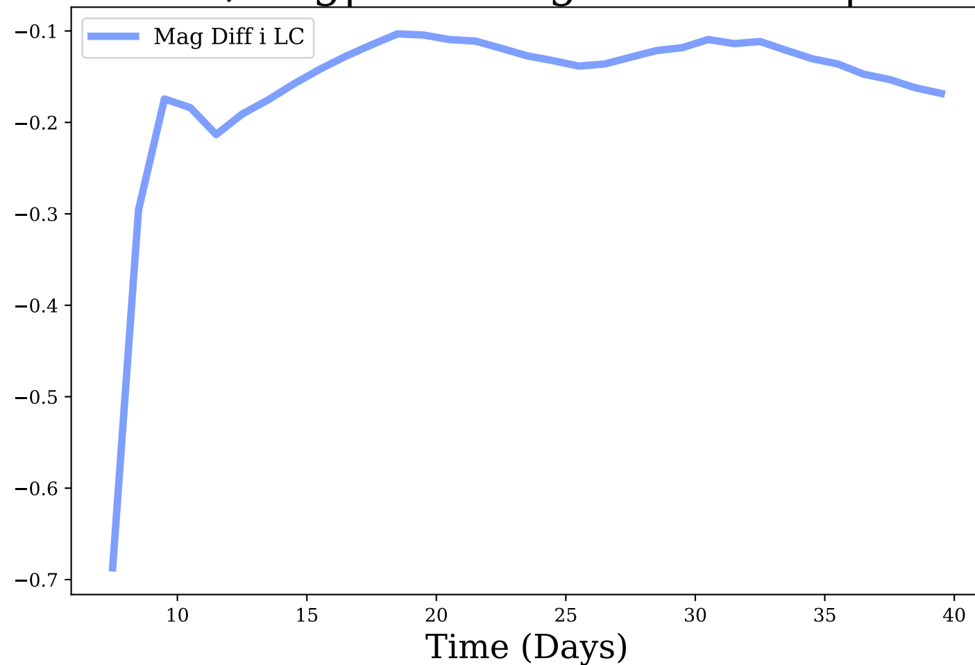
i-band, Avg|Max Mag Diff: -0.16 | 0.69
