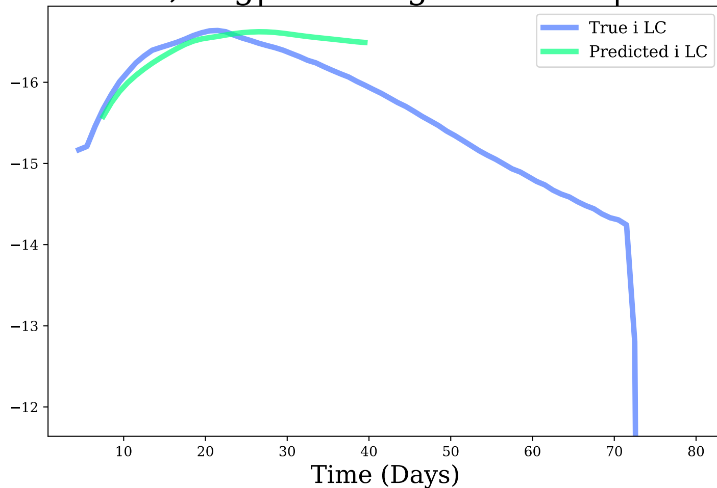
i-band, Avg|Max Mag Diff: 0.19 | 0.53
