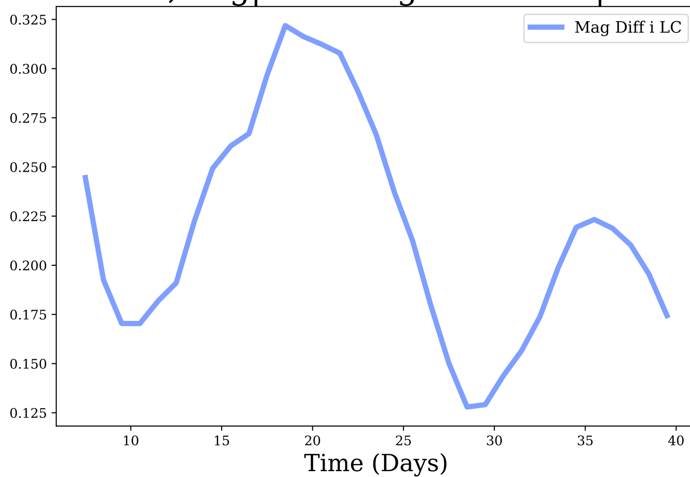
i-band, Avg|Max Mag Diff: 0.22 | 0.32
