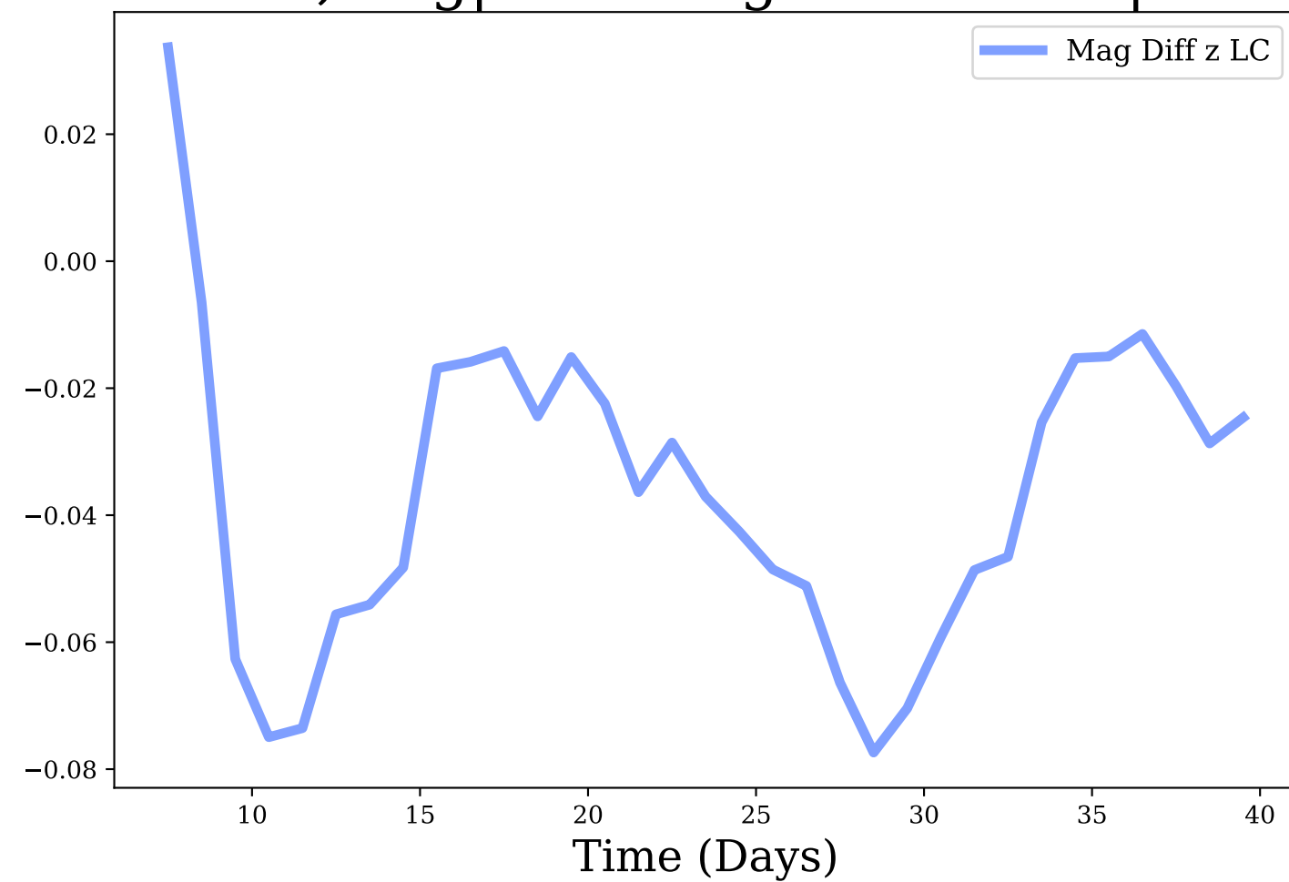
z-band, Avg|Max Mag Diff: -0.04 | 0.08
