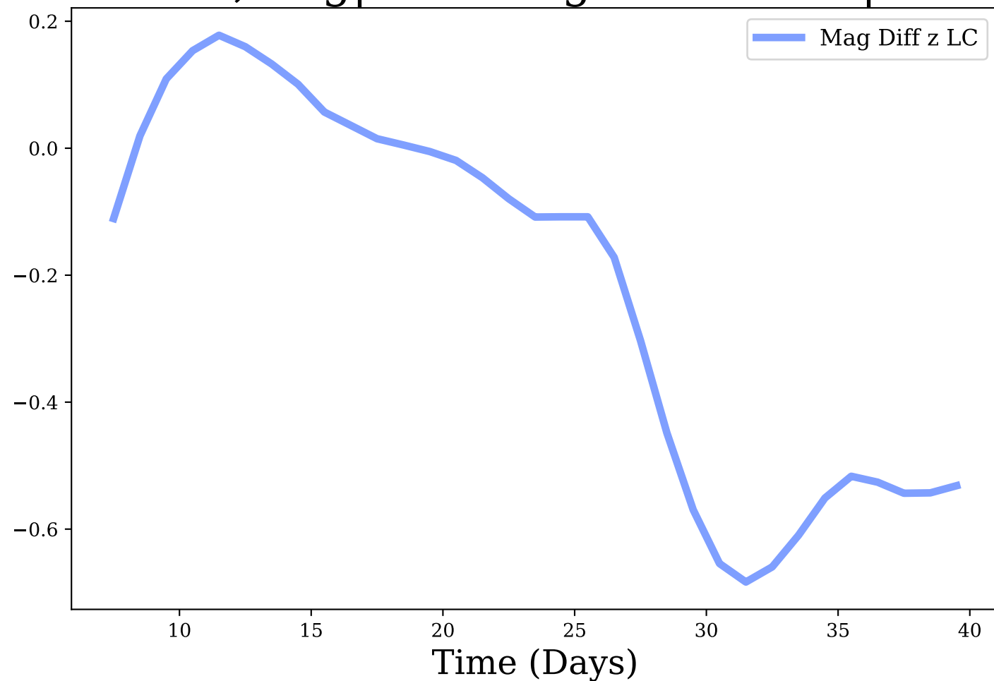
z-band, Avg|Max Mag Diff: -0.21 | 0.68
