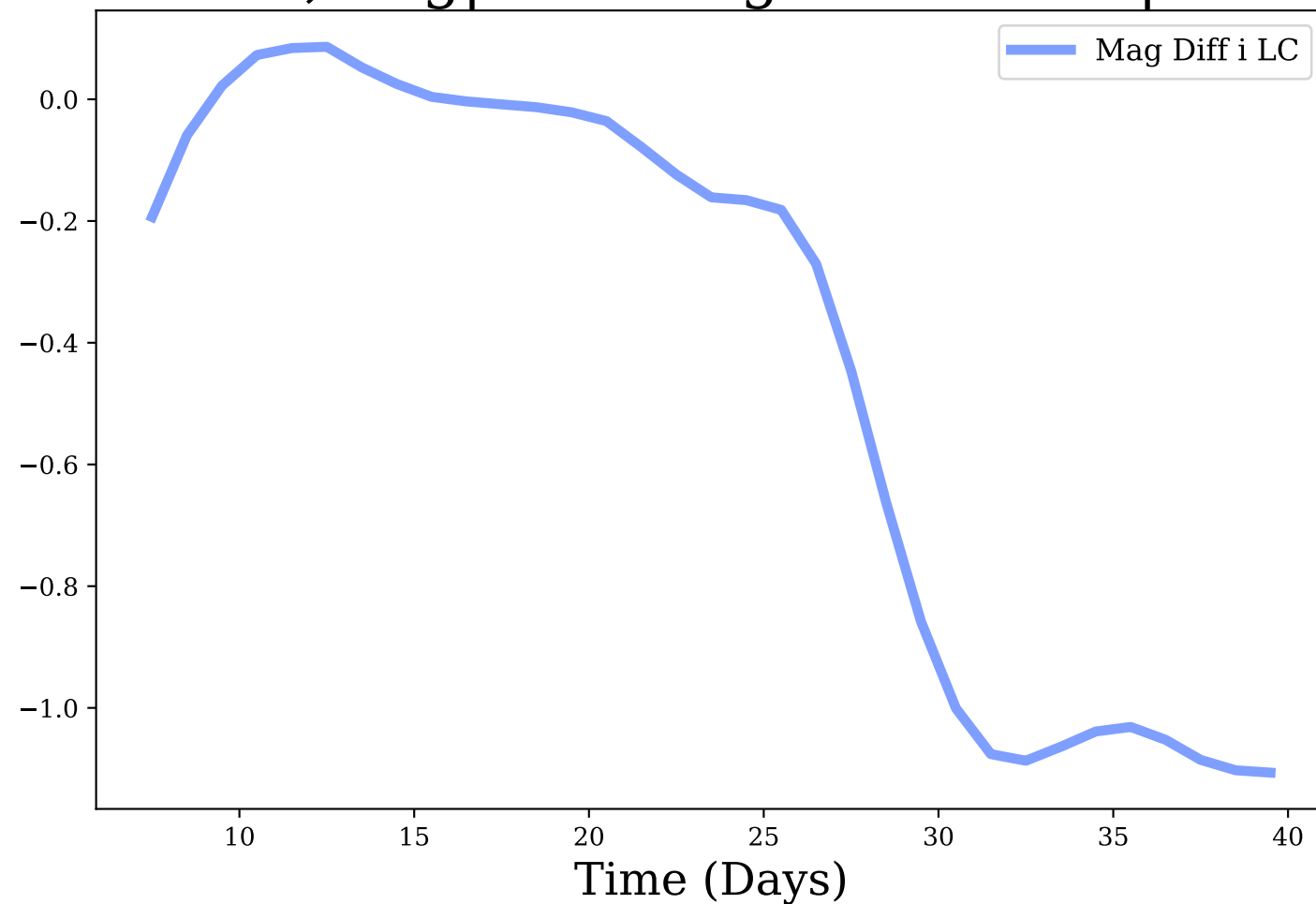
i-band, Avg|Max Mag Diff: -0.41 | 1.11
