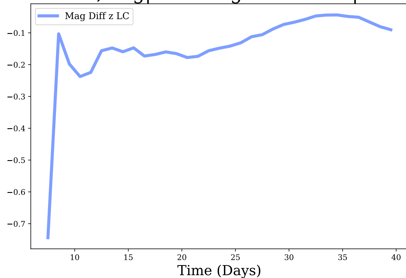
z-band, Avg|Max Mag Diff: -0.14 | 0.74
