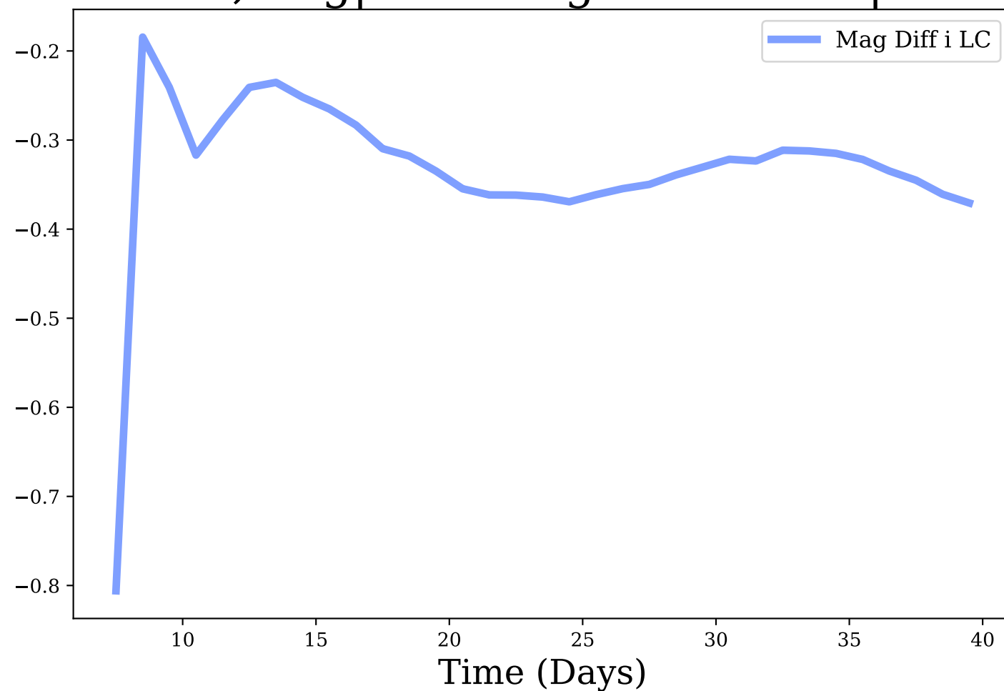
i-band, Avg|Max Mag Diff: -0.33 | 0.81
