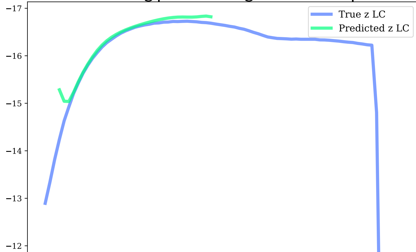
z-band, Avg|Max Mag Diff: 0.1 | 1.04
