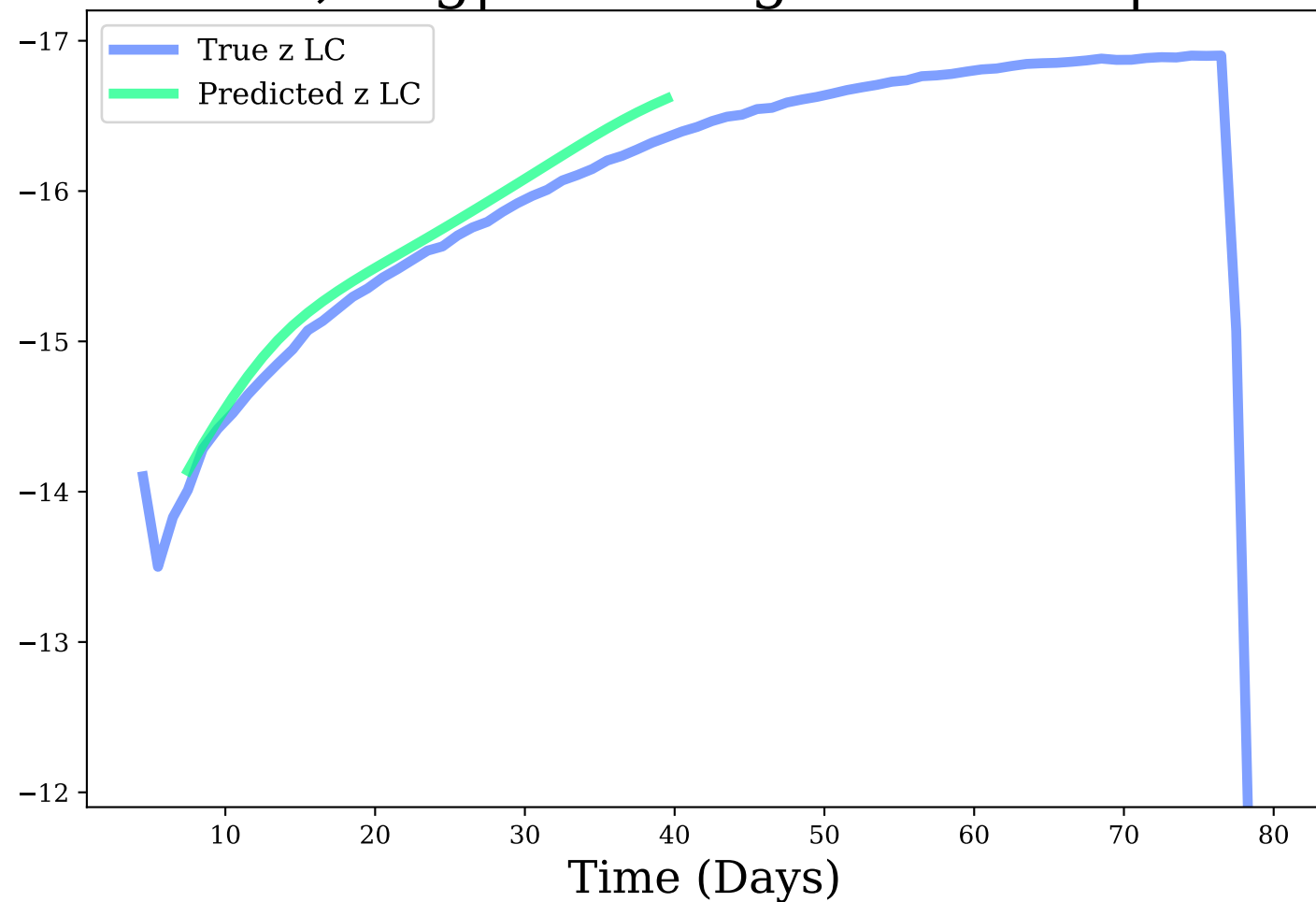
z-band, Avg|Max Mag Diff: 0.14 | 0.26
