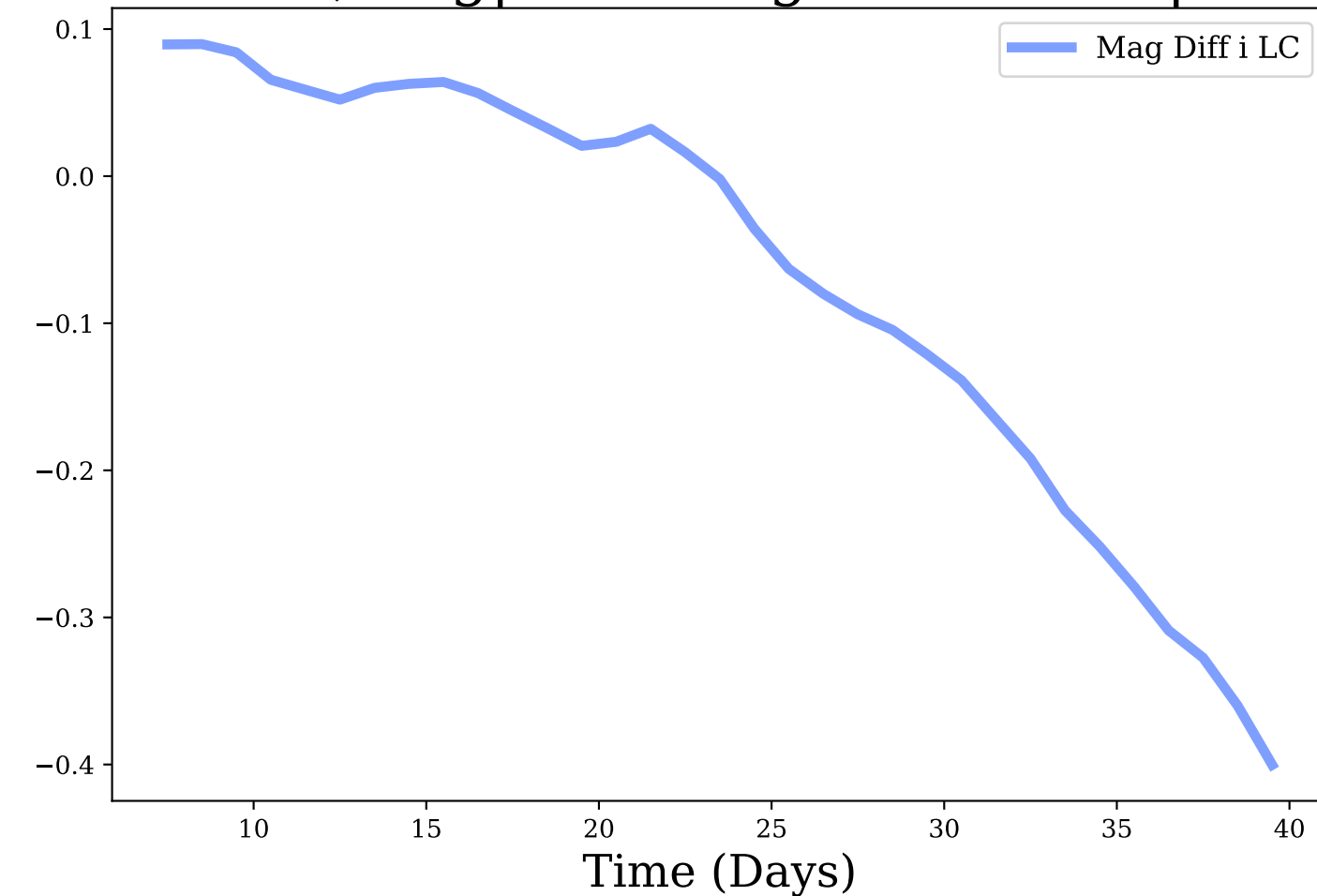
i-band, Avg|Max Mag Diff: -0.07 | 0.4
