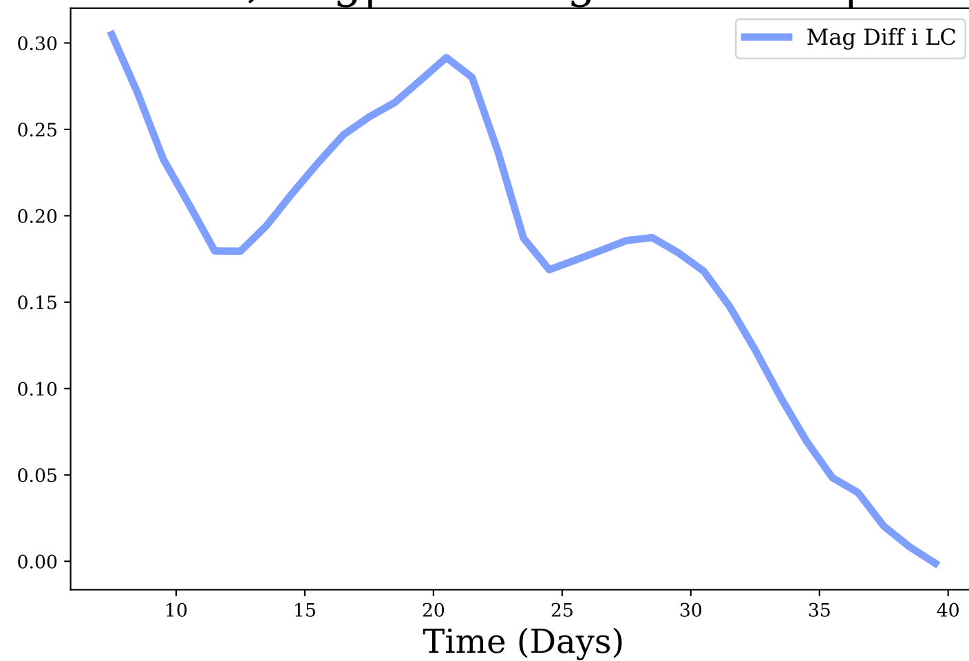
i-band, Avg|Max Mag Diff: 0.18 | 0.3
