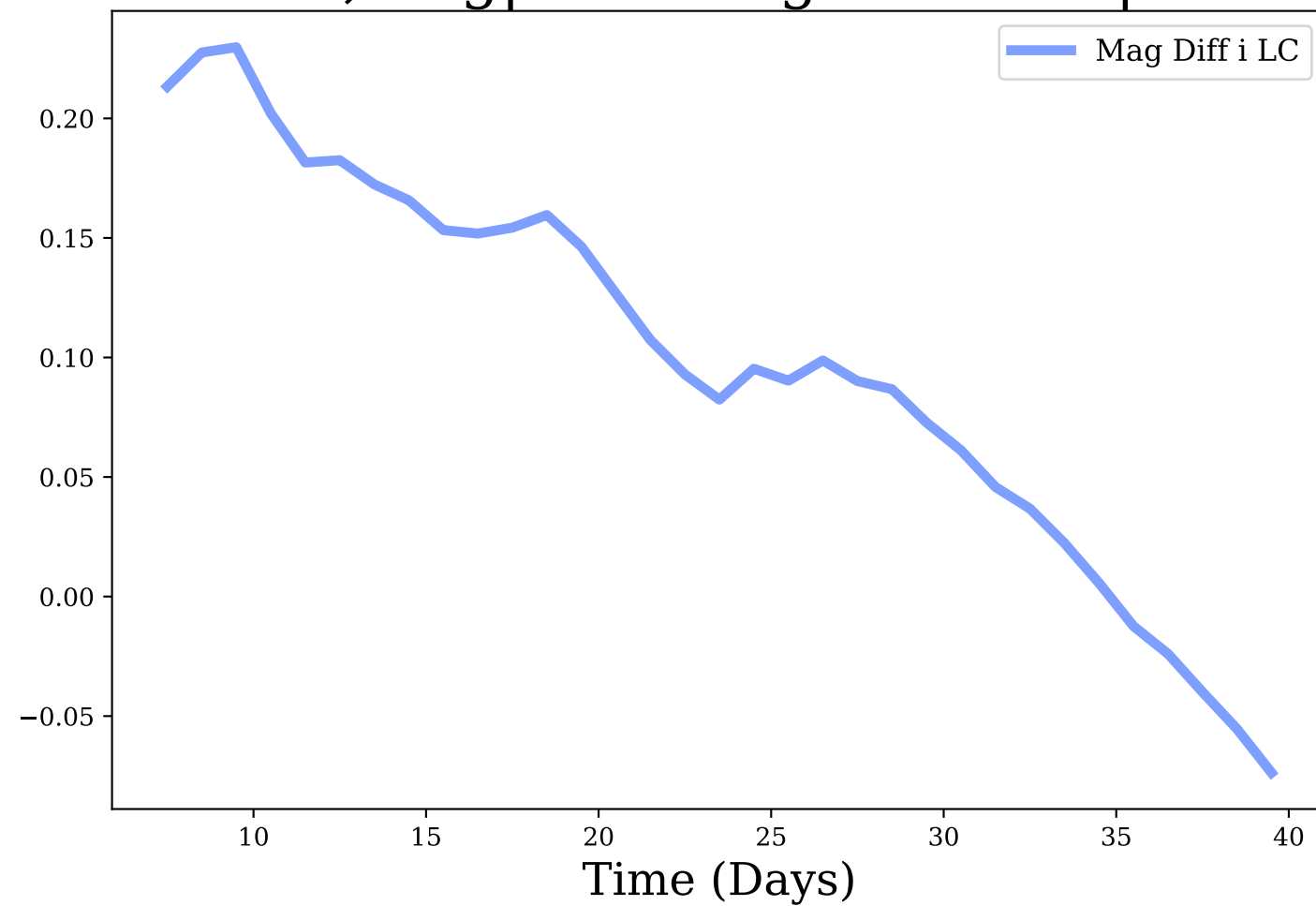
i-band, Avg|Max Mag Diff: 0.1 | 0.23
