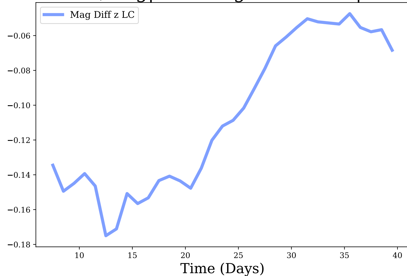
z-band, Avg|Max Mag Diff: -0.11 | 0.18
