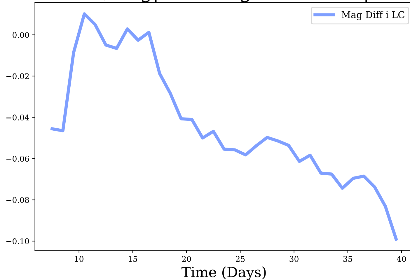
i-band, Avg|Max Mag Diff: -0.04 | 0.1
