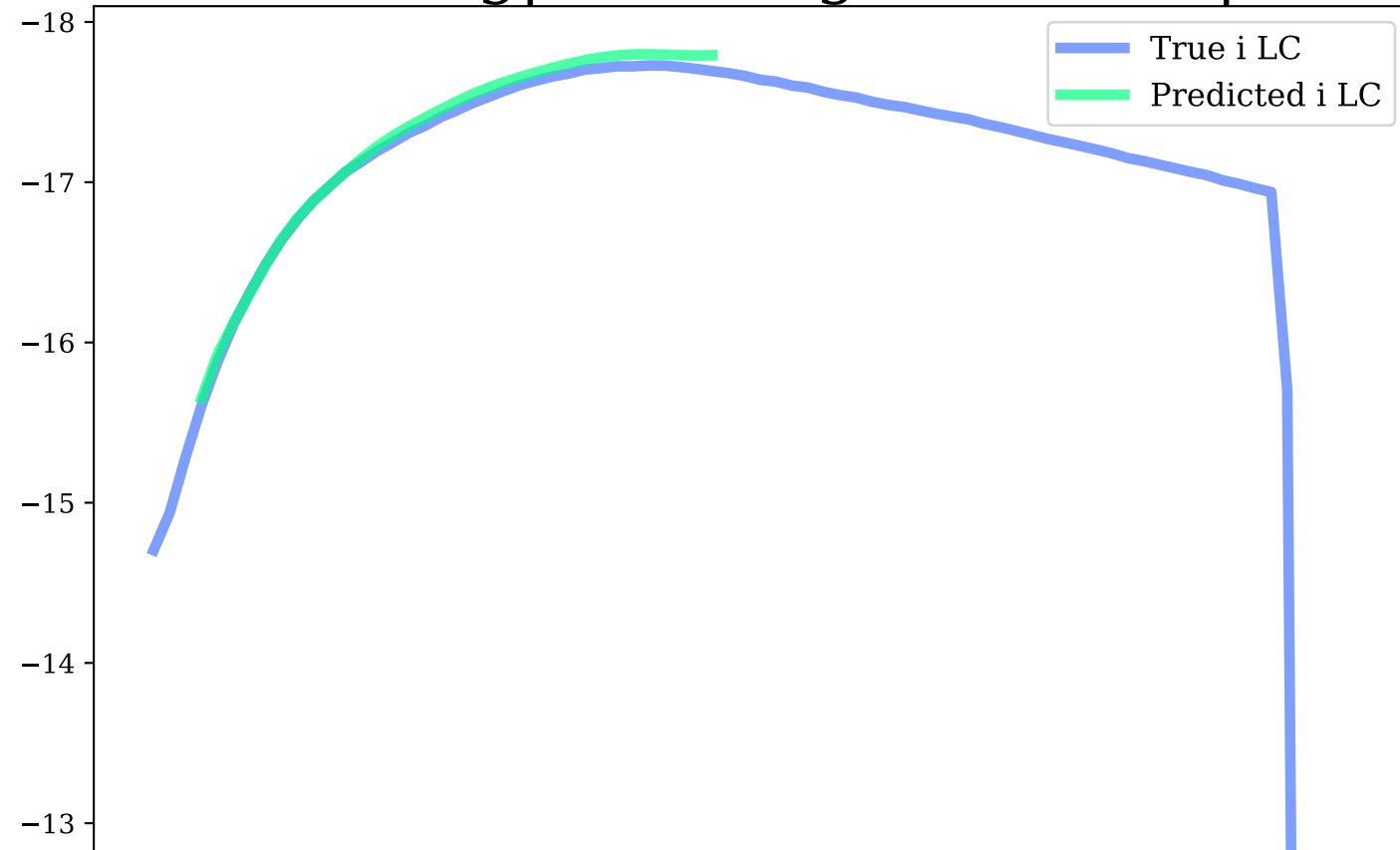
i-band, Avg|Max Mag Diff: 0.04 | 0.1
