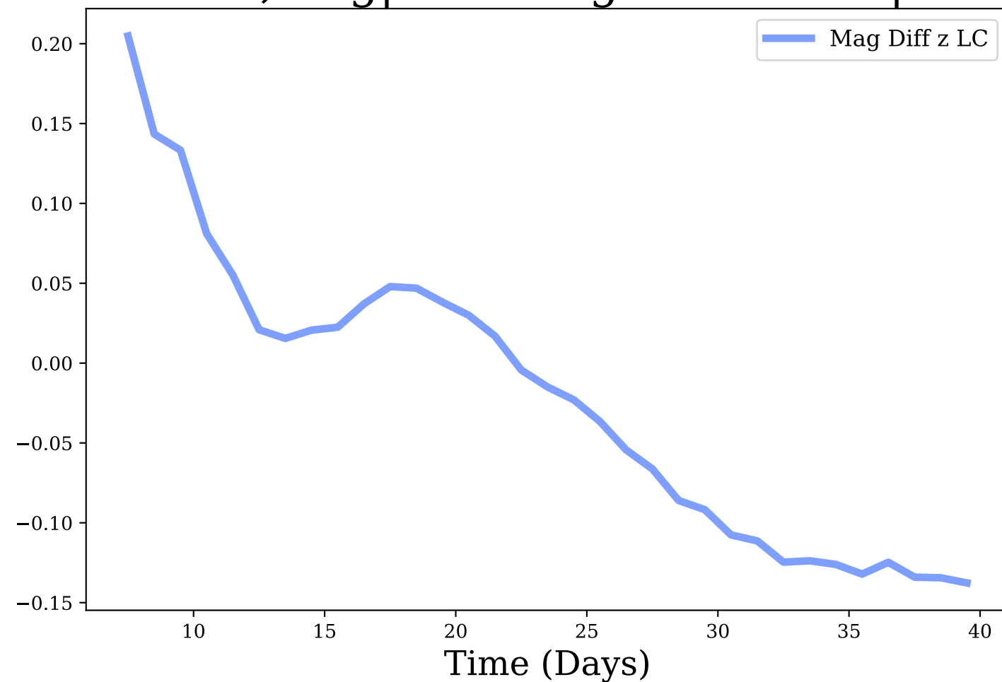
z-band, Avg|Max Mag Diff: -0.02 | 0.2
