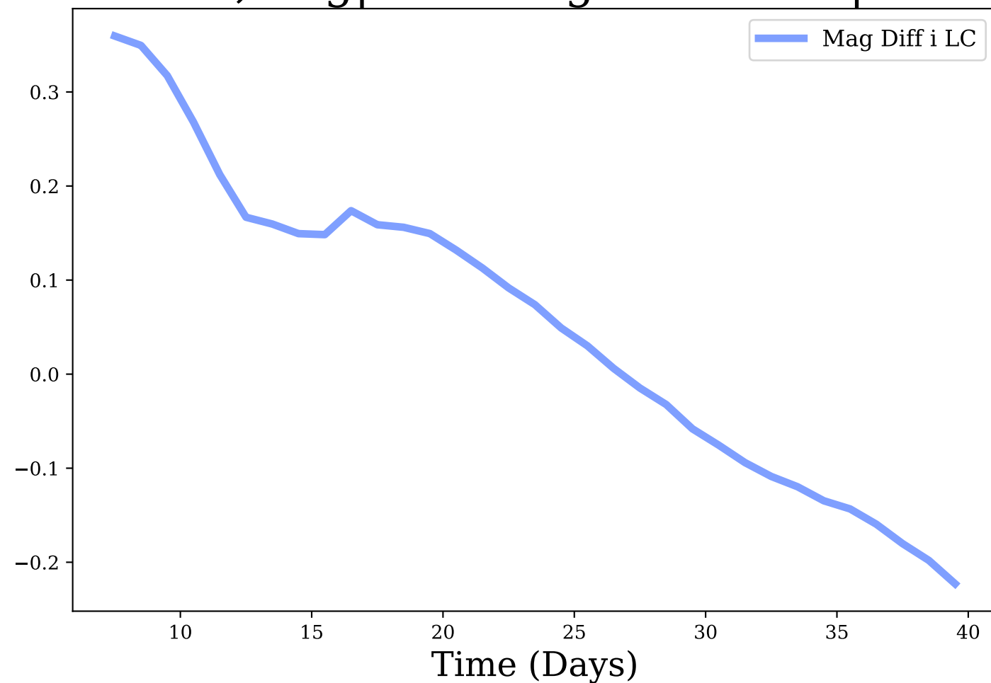
i-band, Avg|Max Mag Diff: 0.05 | 0.36
