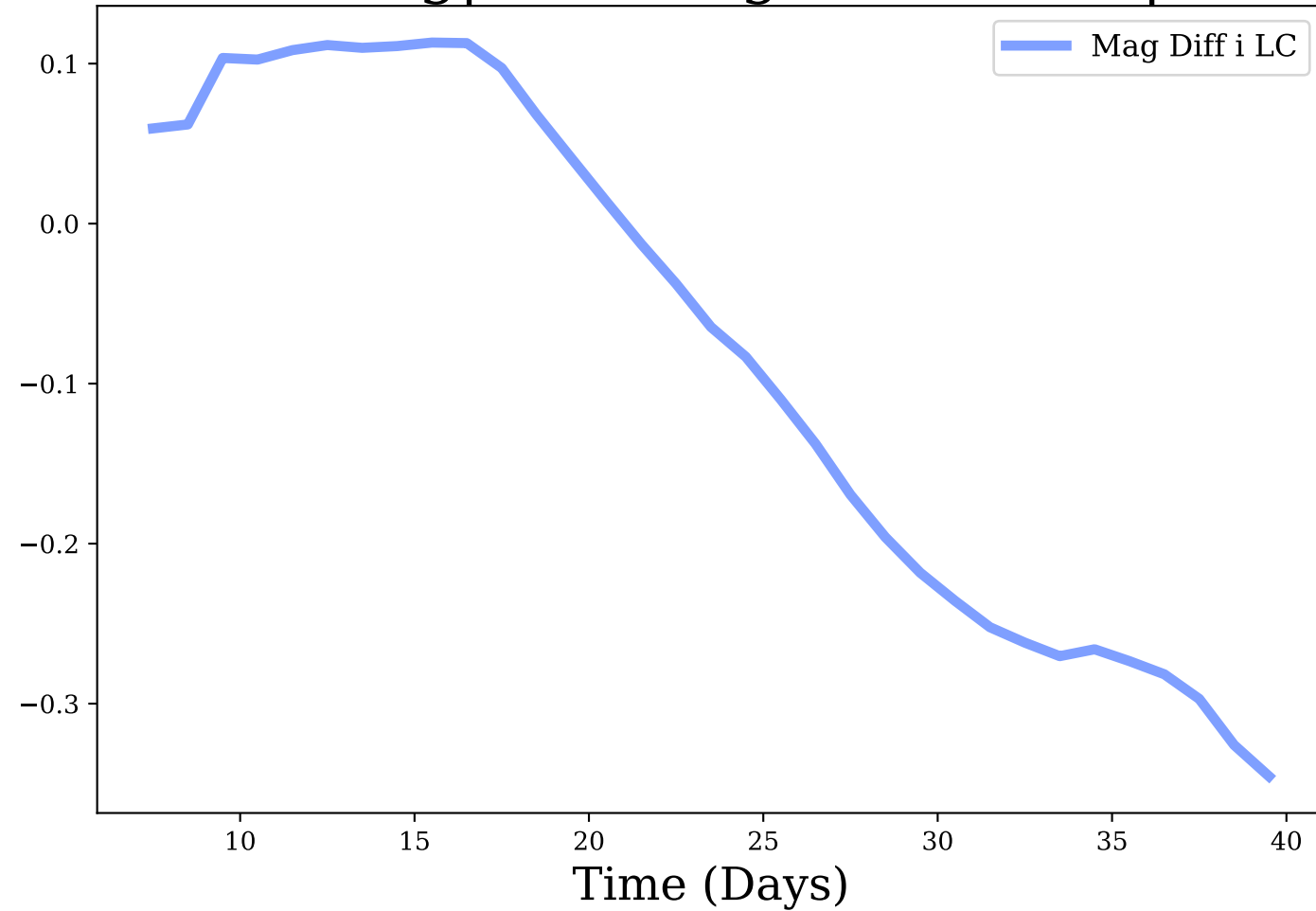
i-band, Avg|Max Mag Diff: -0.08 | 0.35
