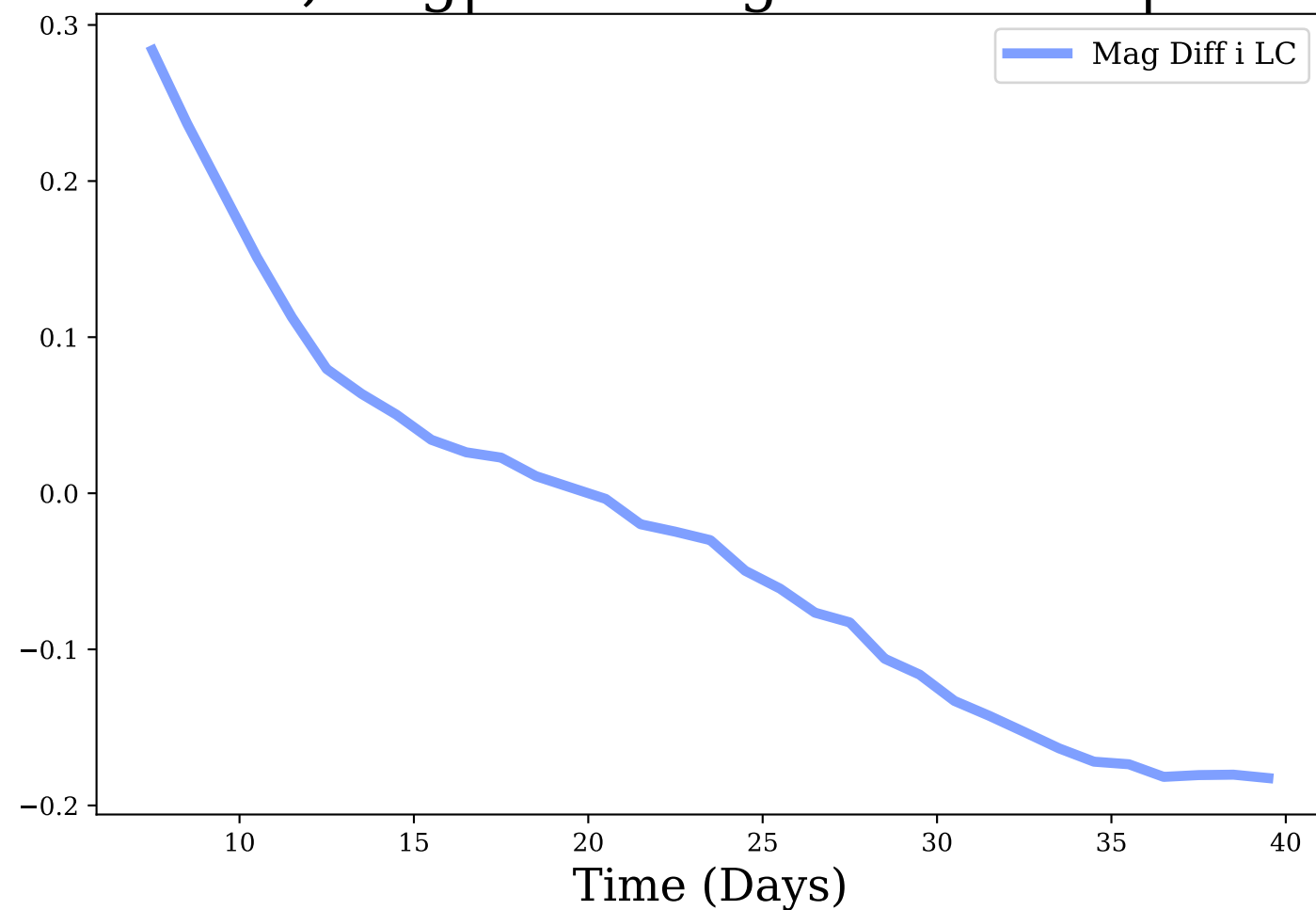
i-band, Avg|Max Mag Diff: -0.03 | 0.28
