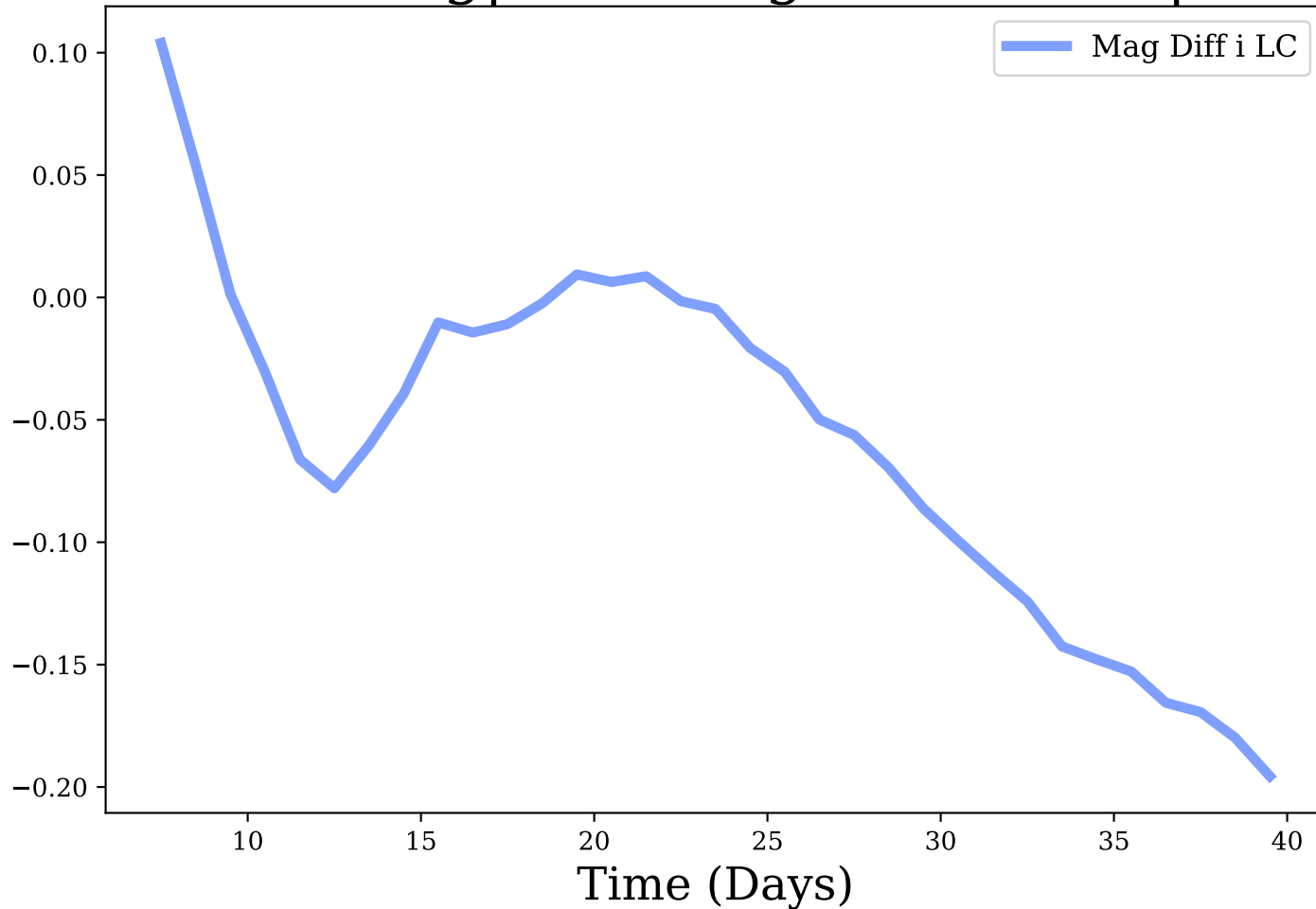
i-band, Avg|Max Mag Diff: -0.06 | 0.2
