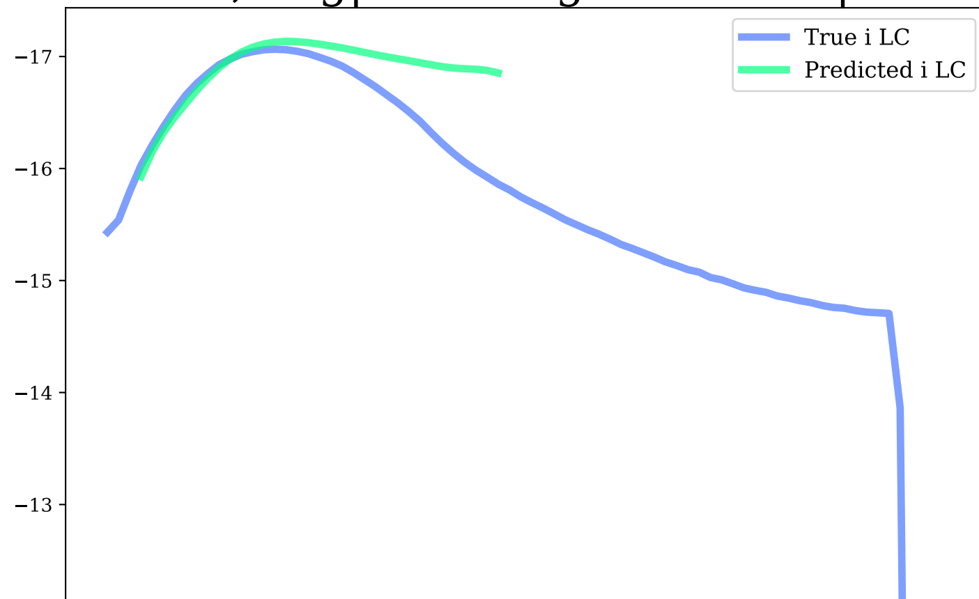
i-band, Avg|Max Mag Diff: 0.29 | 0.99
