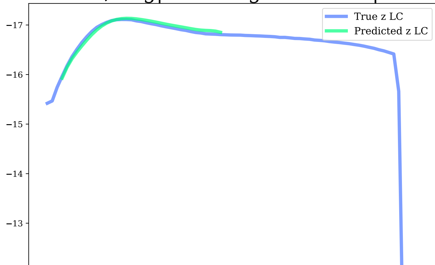
z-band, Avg|Max Mag Diff: 0.05 | 0.07
