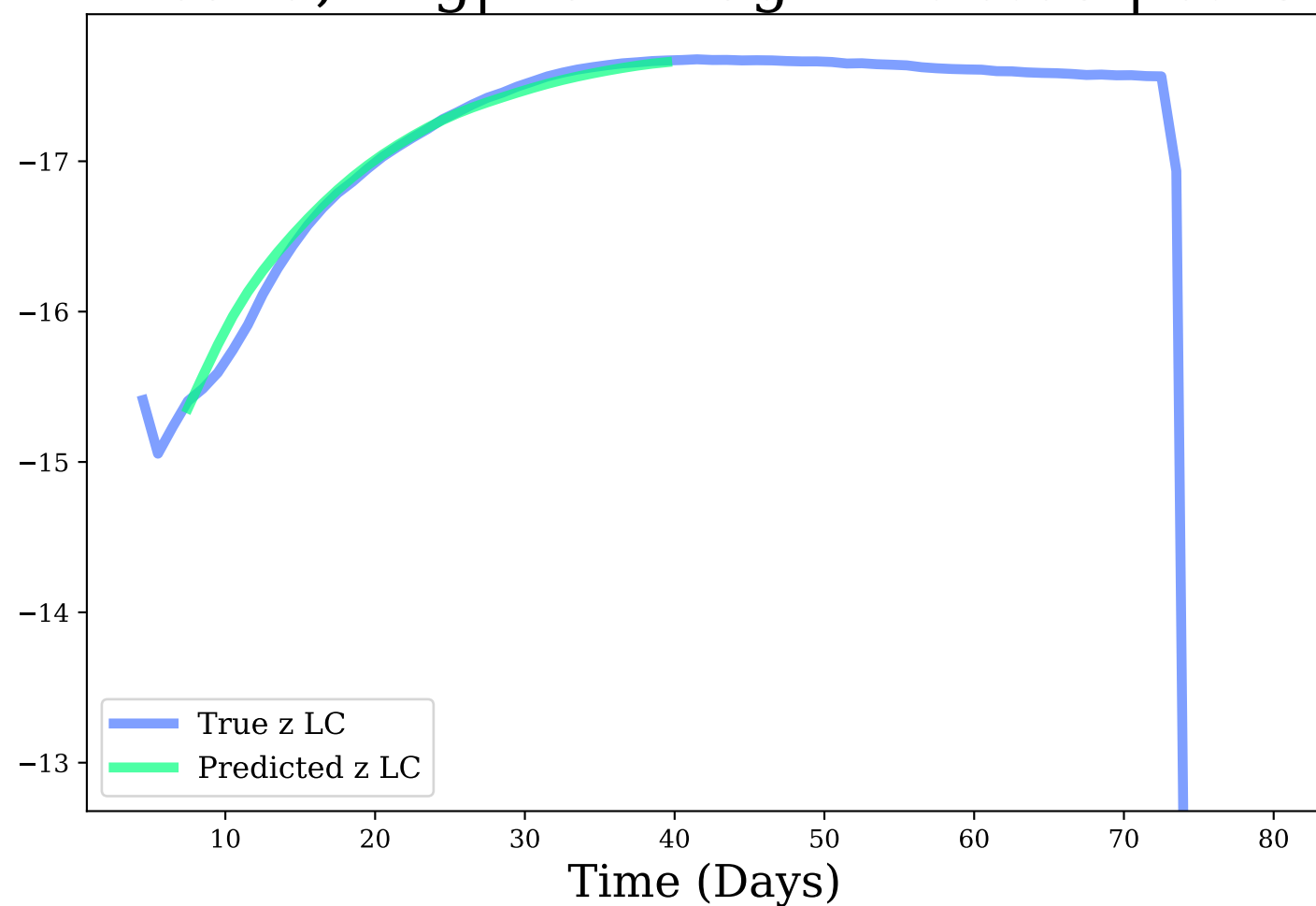
z-band, Avg|Max Mag Diff: 0.05 | 0.23
