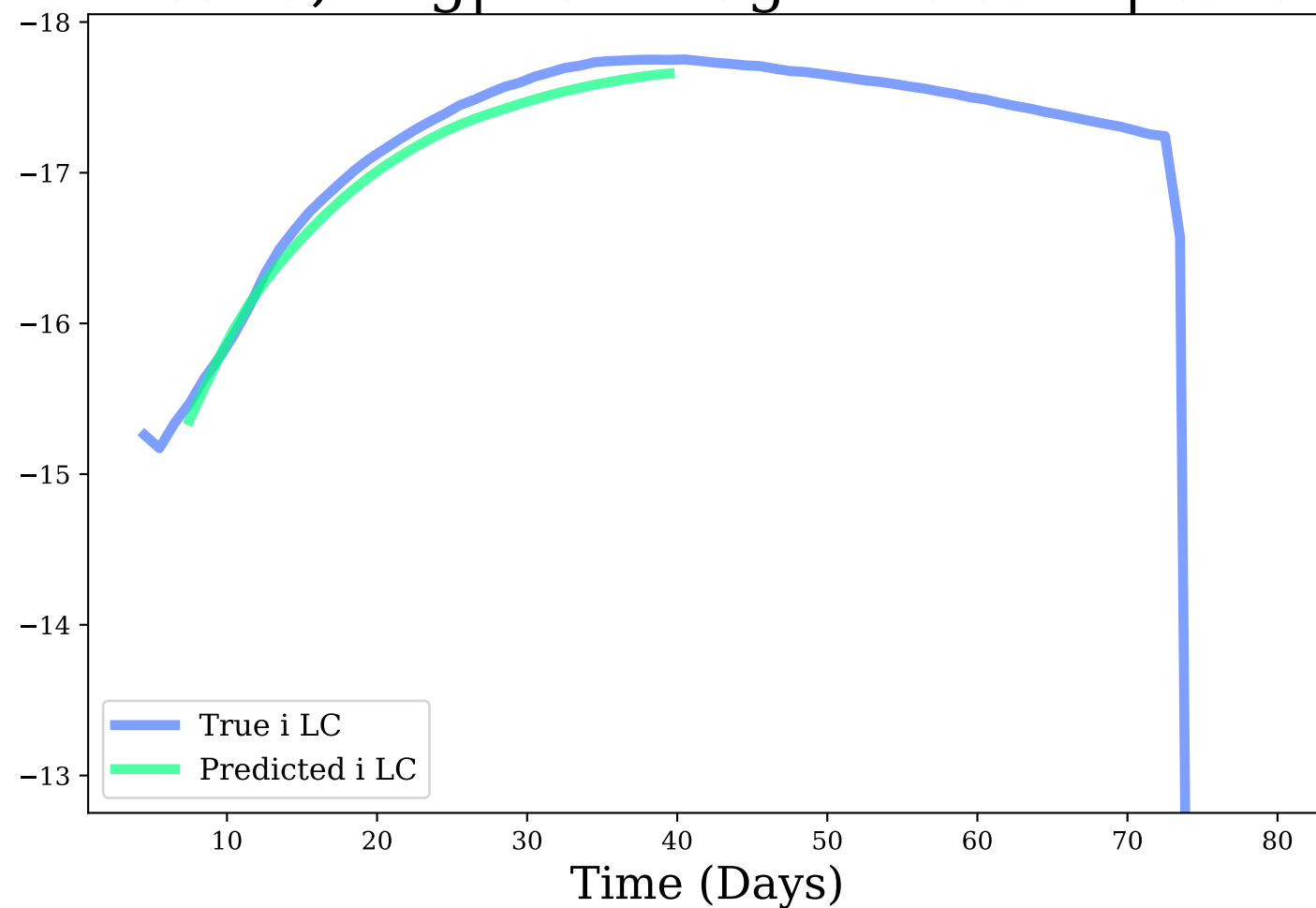
i-band, Avg|Max Mag Diff: 0.11 | 0.15
