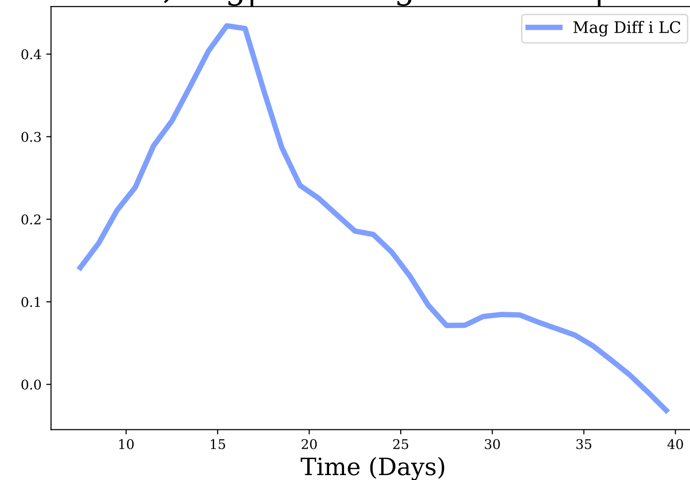
i-band, Avg|Max Mag Diff: 0.17 | 0.43
