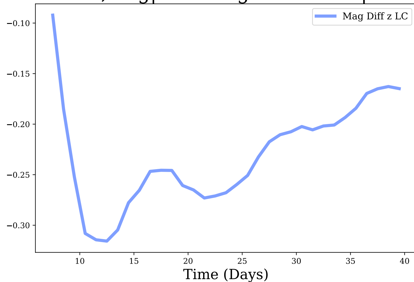
z-band, Avg|Max Mag Diff: -0.23 | 0.32
