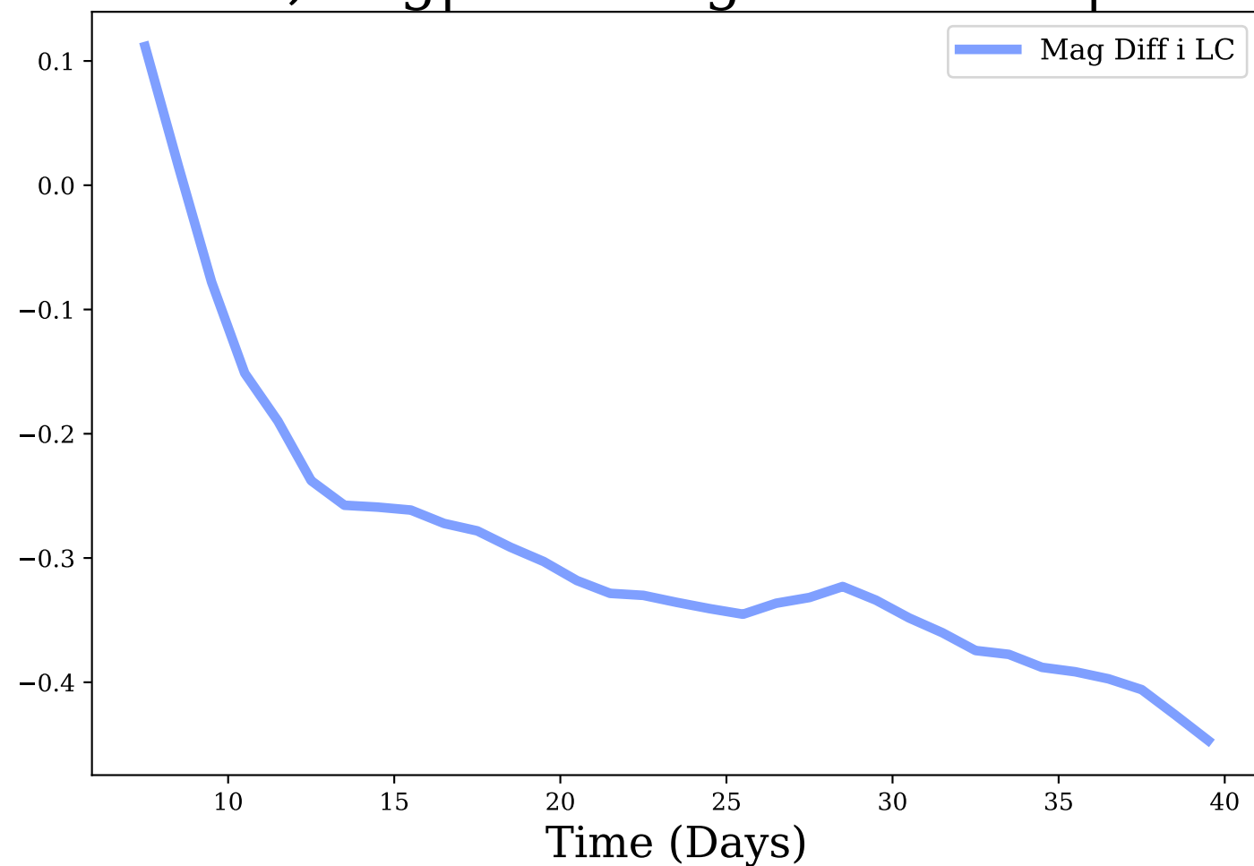
i-band, Avg|Max Mag Diff: -0.29 | 0.45
