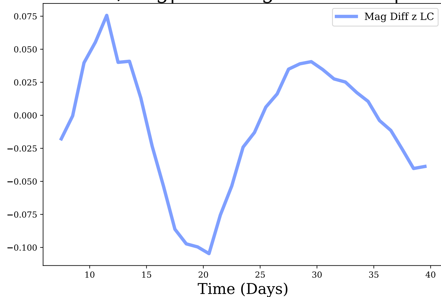
z-band, Avg|Max Mag Diff: -0.01 | 0.1
