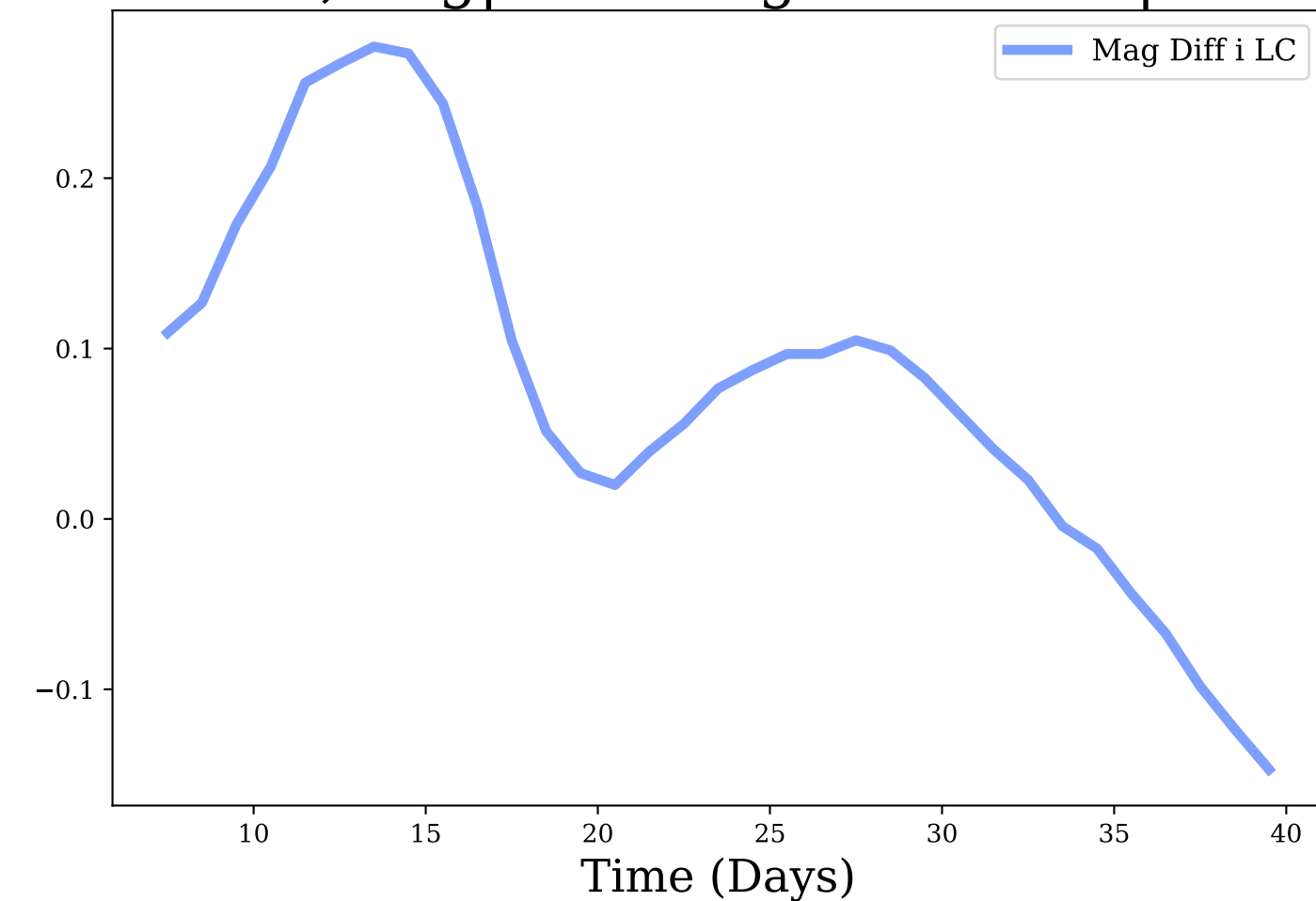
i-band, Avg|Max Mag Diff: 0.08 | 0.28
