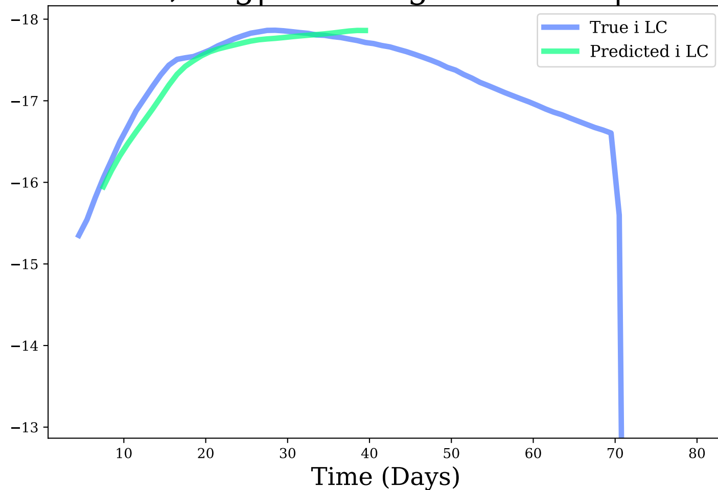
i-band, Avg|Max Mag Diff: 0.11 | 0.28
