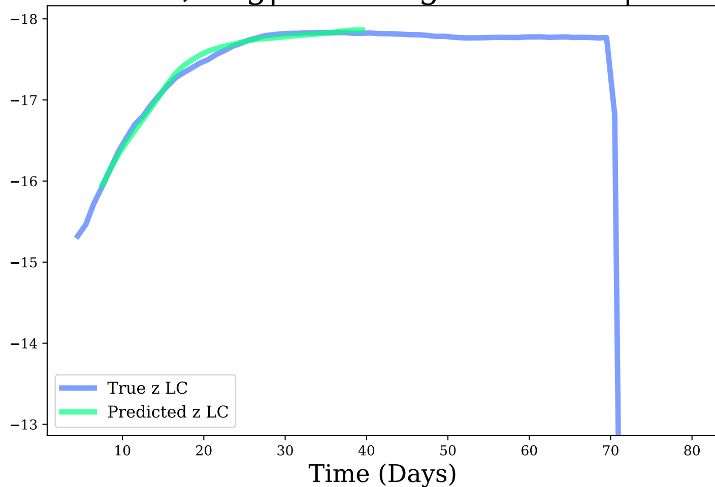
z-band, Avg|Max Mag Diff: 0.04 | 0.1
