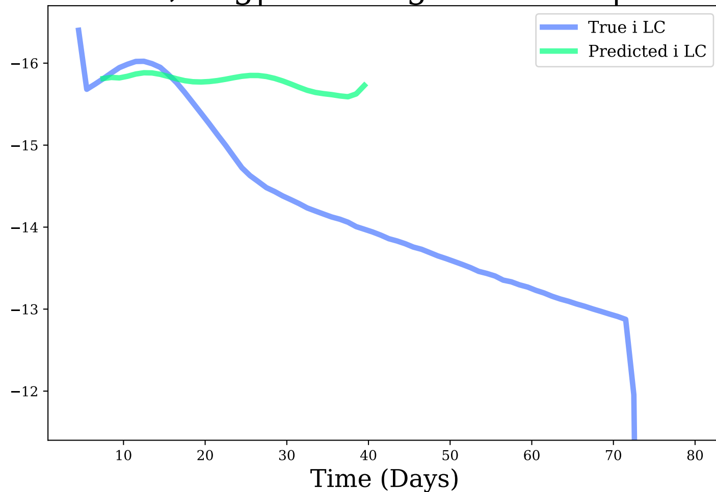
i-band, Avg|Max Mag Diff: 0.83 | 1.75
