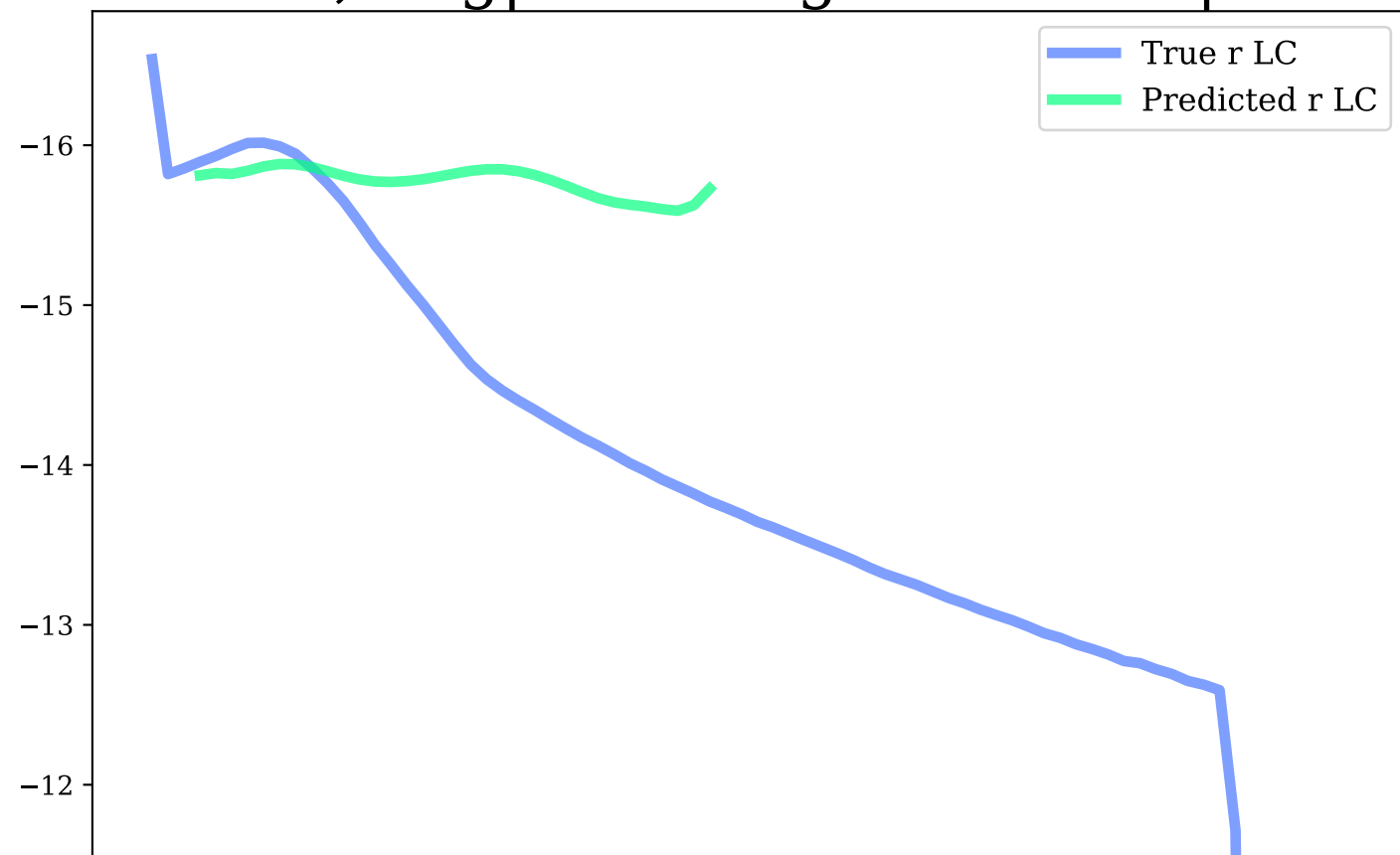
z-band, Avg|Max Mag Diff: 0.34 | 0.68
