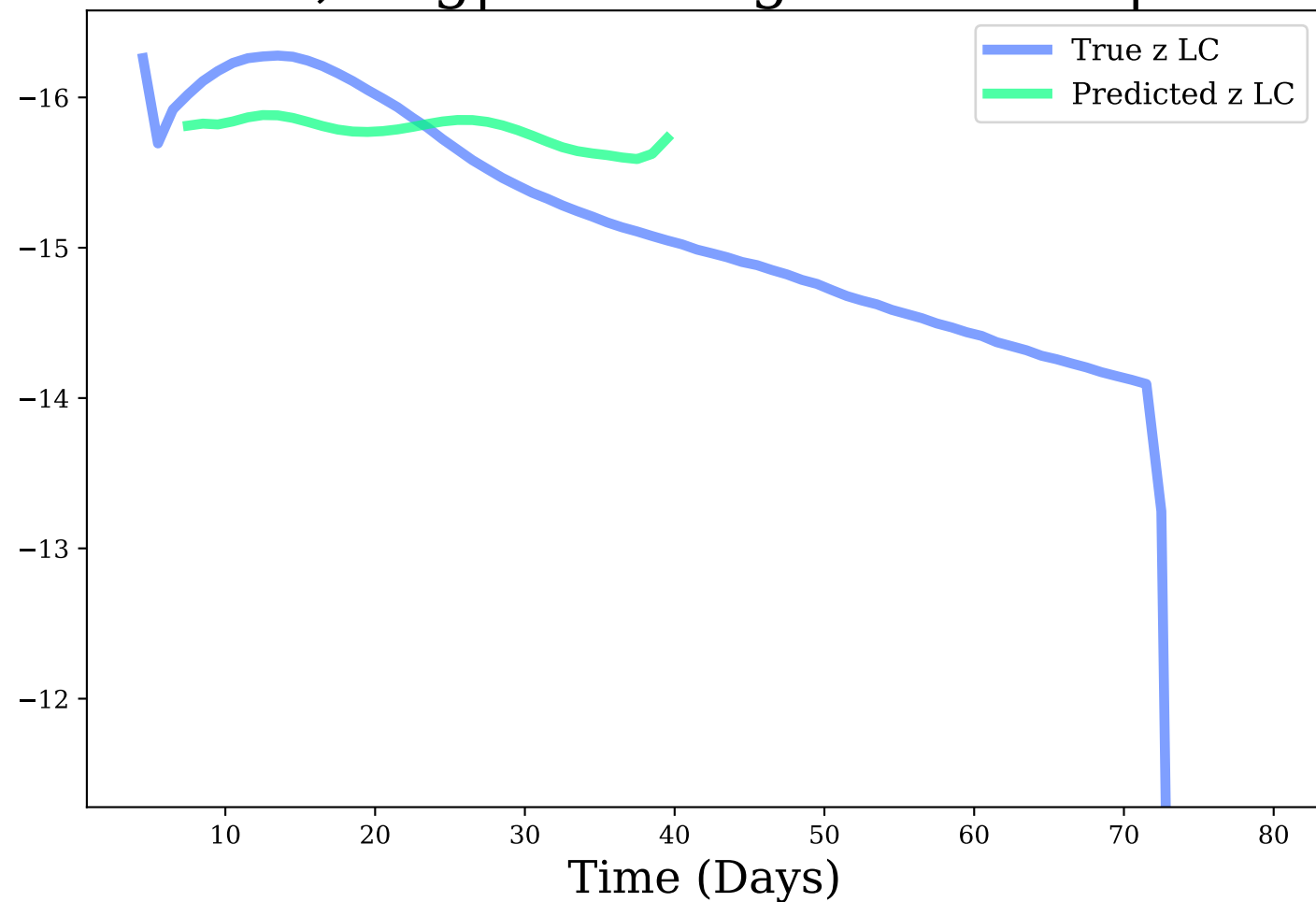
z-band, Avg|Max Mag Diff: 0.34 | 0.68
