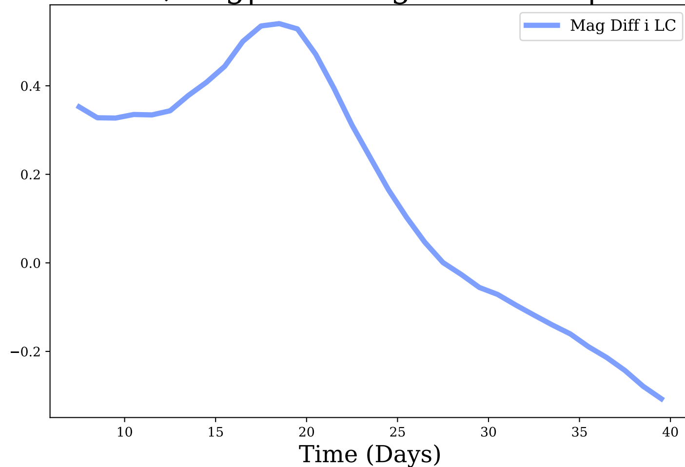
i-band, Avg|Max Mag Diff: 0.16 | 0.54
