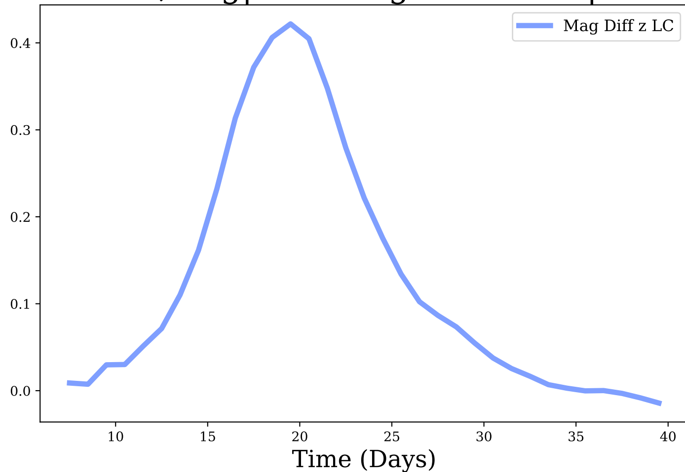
z-band, Avg|Max Mag Diff: 0.13 | 0.42
