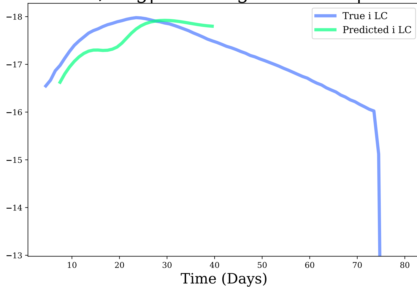
i-band, Avg|Max Mag Diff: 0.27 | 0.54
