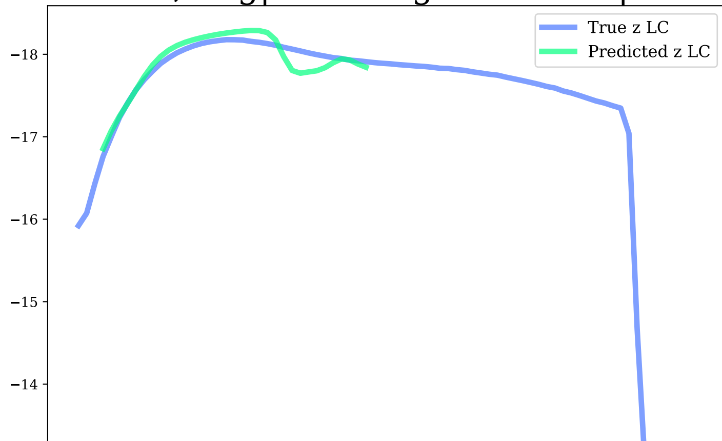
z-band, Avg|Max Mag Diff: 0.09 | 0.27
