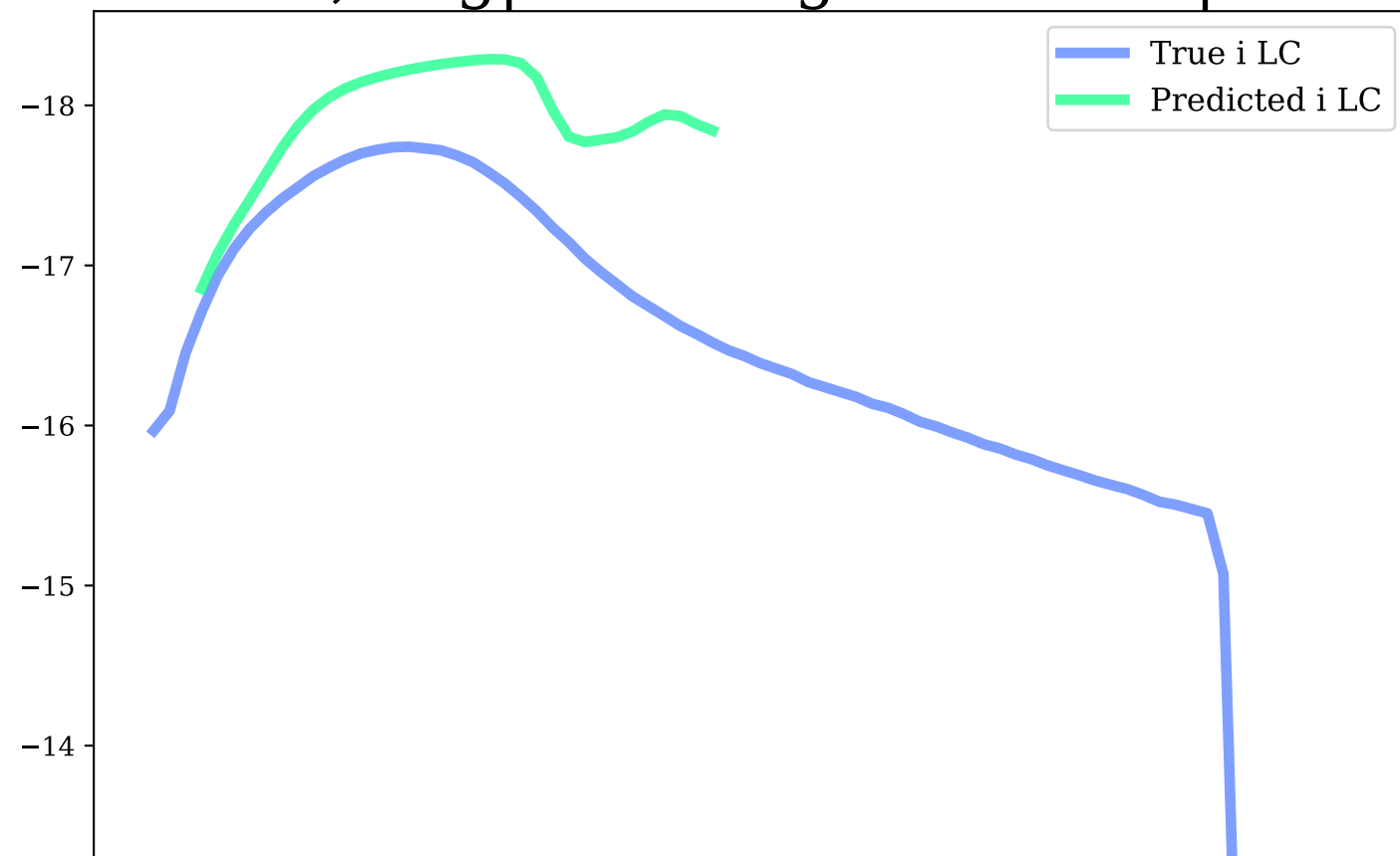
i-band, Avg|Max Mag Diff: 0.65 | 1.32
