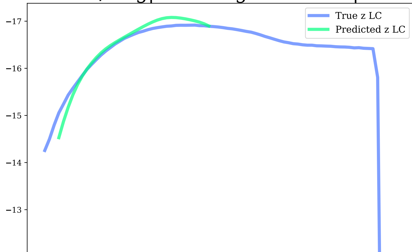
z-band, Avg|Max Mag Diff: 0.11 | 0.53
