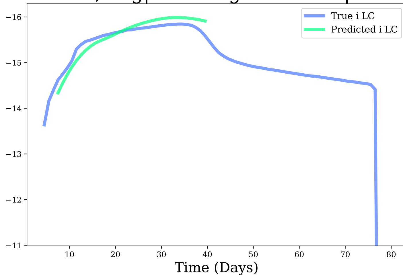
i-band, Avg|Max Mag Diff: 0.14 | 0.32
