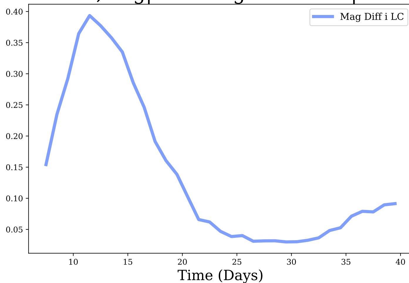
i-band, Avg|Max Mag Diff: 0.14 | 0.39
