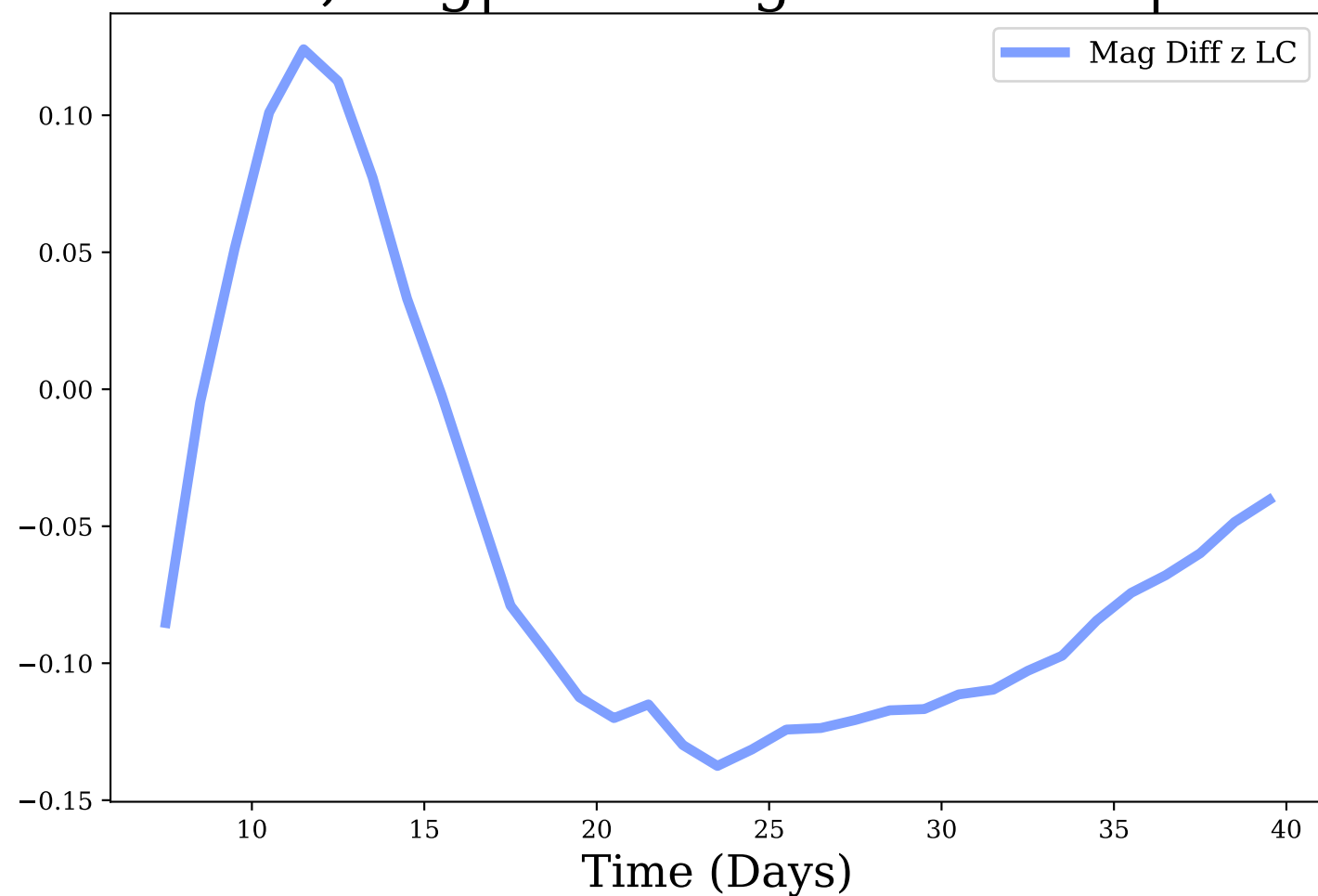
z-band, Avg|Max Mag Diff: -0.06 | 0.14
