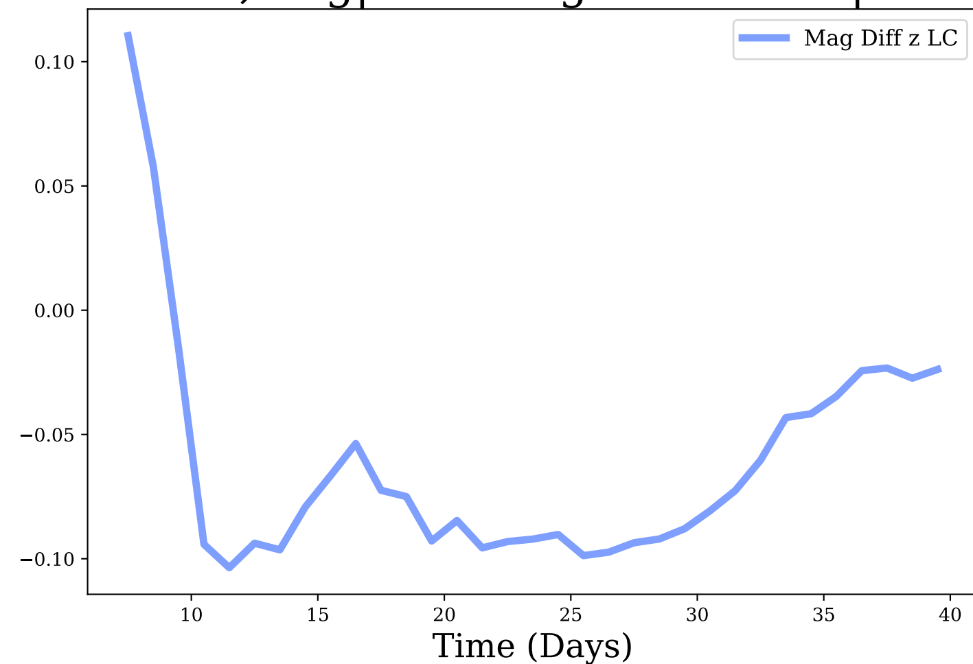
z-band, Avg|Max Mag Diff: -0.06 | 0.11
