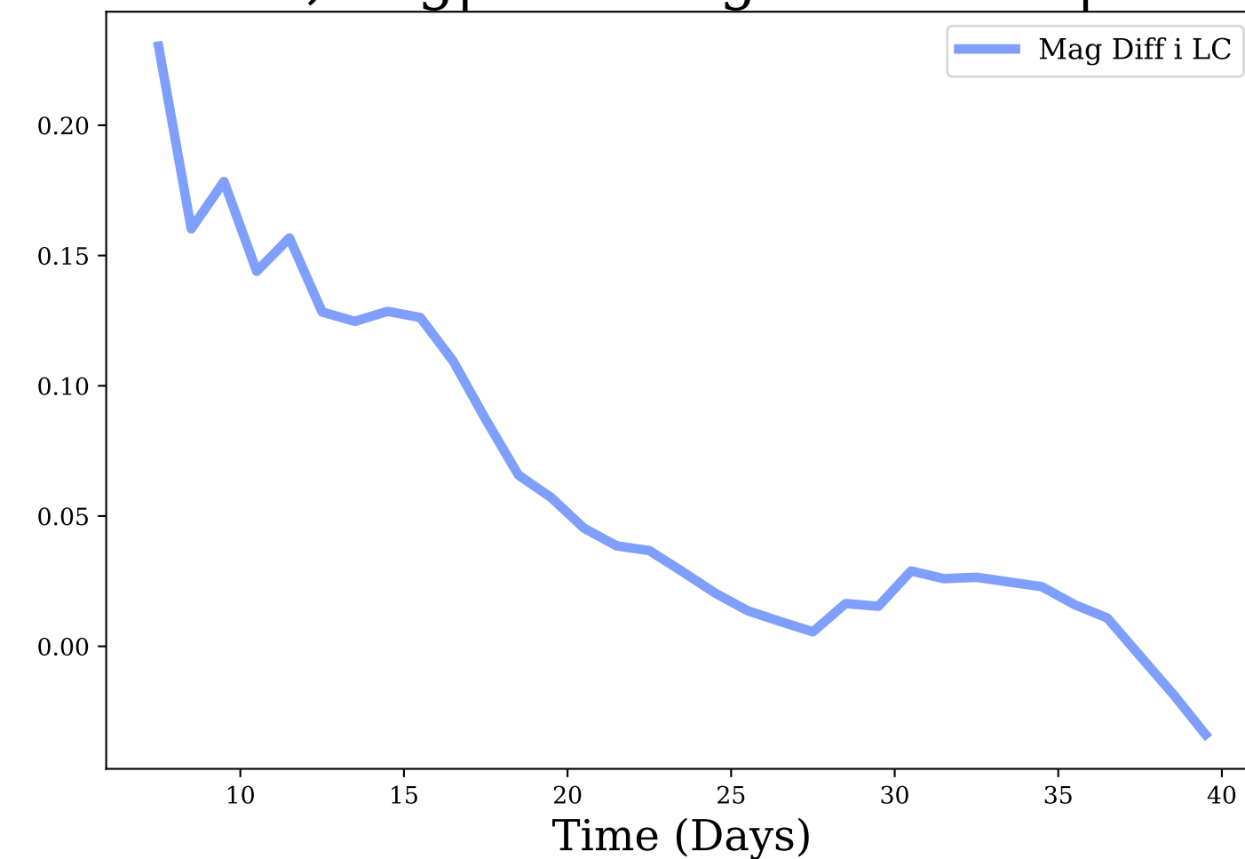
i-band, Avg|Max Mag Diff: 0.06 | 0.23
